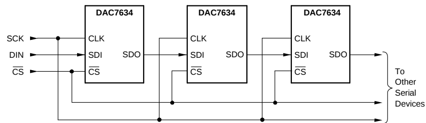
Figure 61. Daisy-Chaining DAC7634
