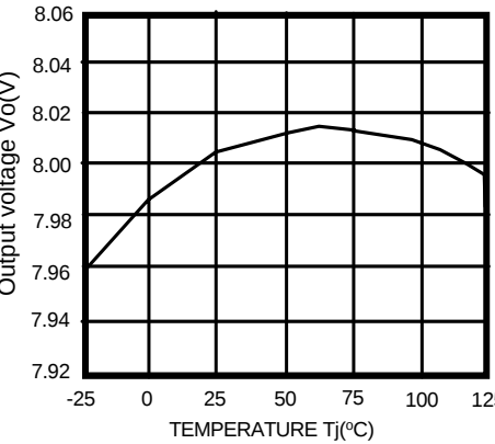
Figure 4. Output Voltage vs. Temperature( T_j )
