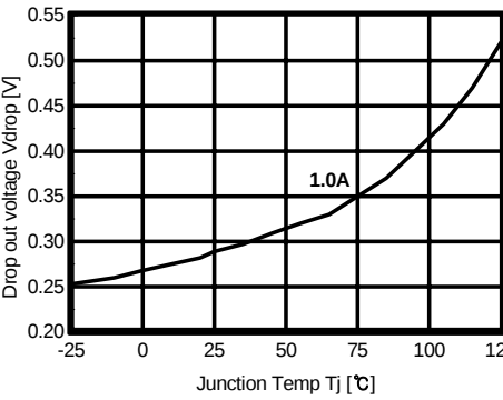
Figure 6. Dropout Voltage vs. Junction Temperature
