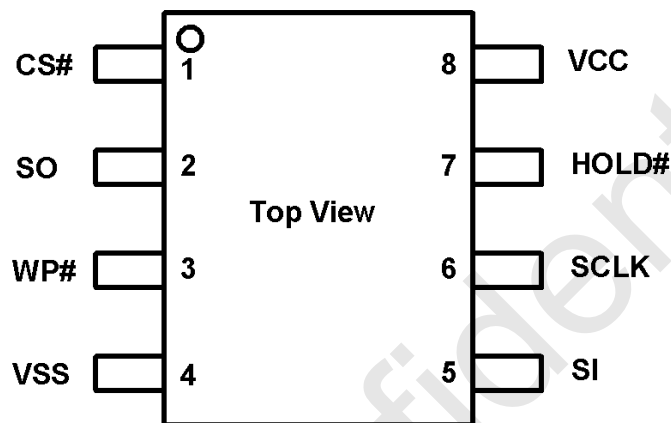
8 – LEAD SOP
