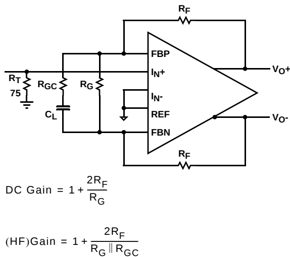
FIGURE 25. TRANSMIT EQUALIZER
