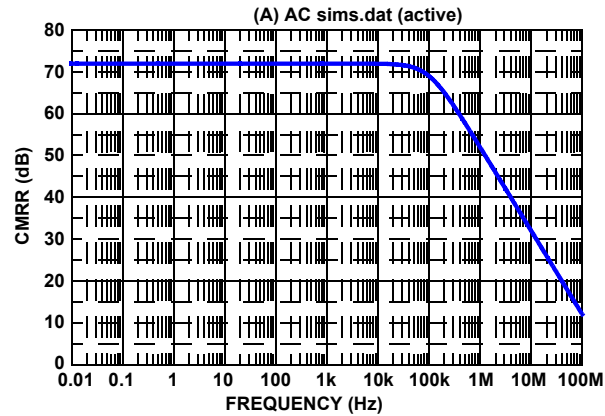
FIGURE 32. SIMULATED (SPICE) CMRR
