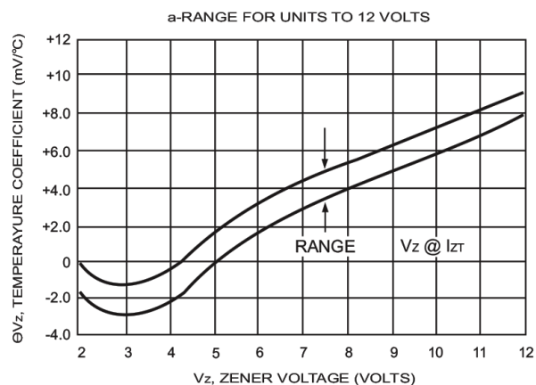
FIG.7- TEMPERATURE COEFFICIENTS
