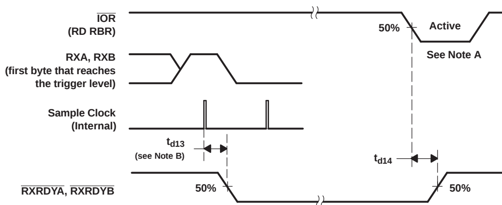
Figure 17. Receiver Ready (RXRDY) Waveforms, FCR0 = 1 and FCR3 = 1 (Mode 1)
