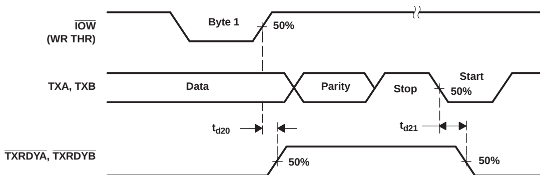
Figure 19. Transmitter Ready ( \overline{\text{TXRDY}} ) Waveforms, FCR0 = 0 or FCR0 = 1 and FCR3 = 0 (Mode 0)
