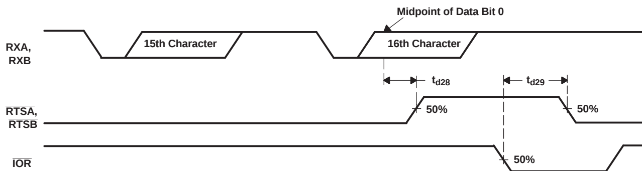
Figure 24. Auto- \overline{\text{RTS}} Timing for RCV Threshold of 14 Waveforms
