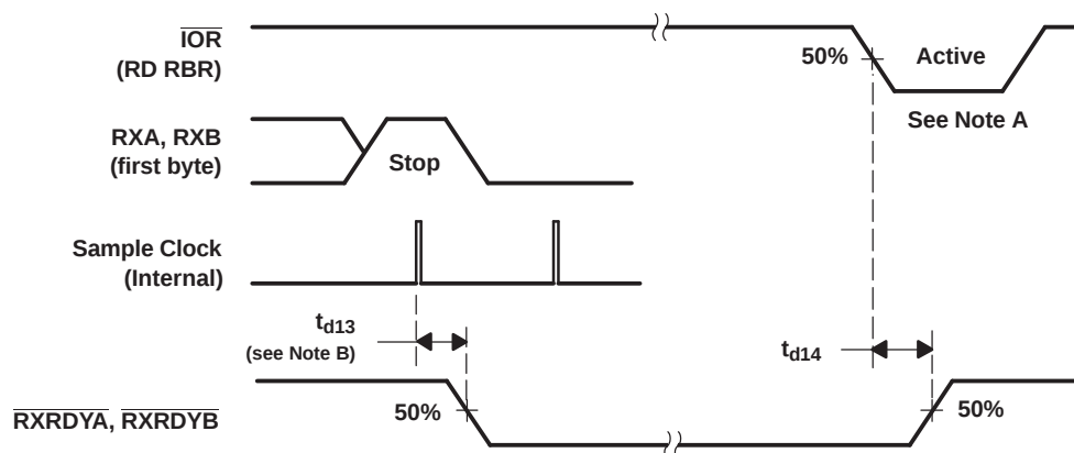
Figure 16. Receiver Ready (RXRDY) Waveforms, FCR0 = 0 or FCR0 = 1 and FCR3 = 0 (Mode 0)
