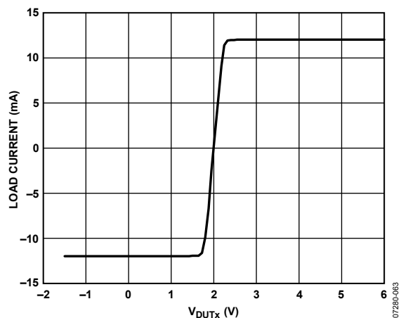
Figure 40. Active Load Commutation Response; V_{COM} = 2.0\text{ V} ; I_{OH} = I_{OL} = 12\text{ mA}
