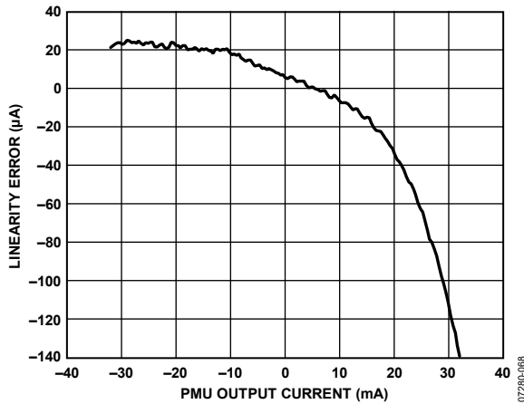
Figure 45. PMU Force Current Range A Linearity
