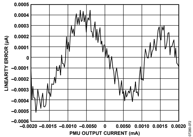
Figure 49. PMU Force Current Range E Linearity
