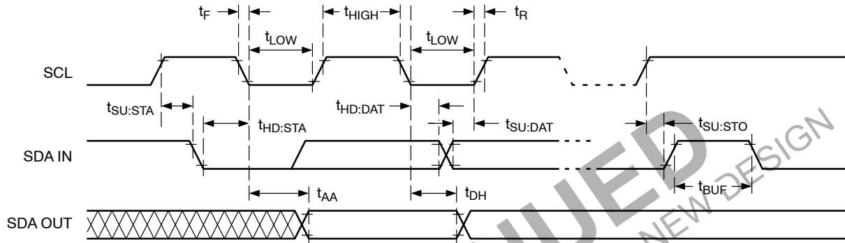
Figure 2. Bus Timing
