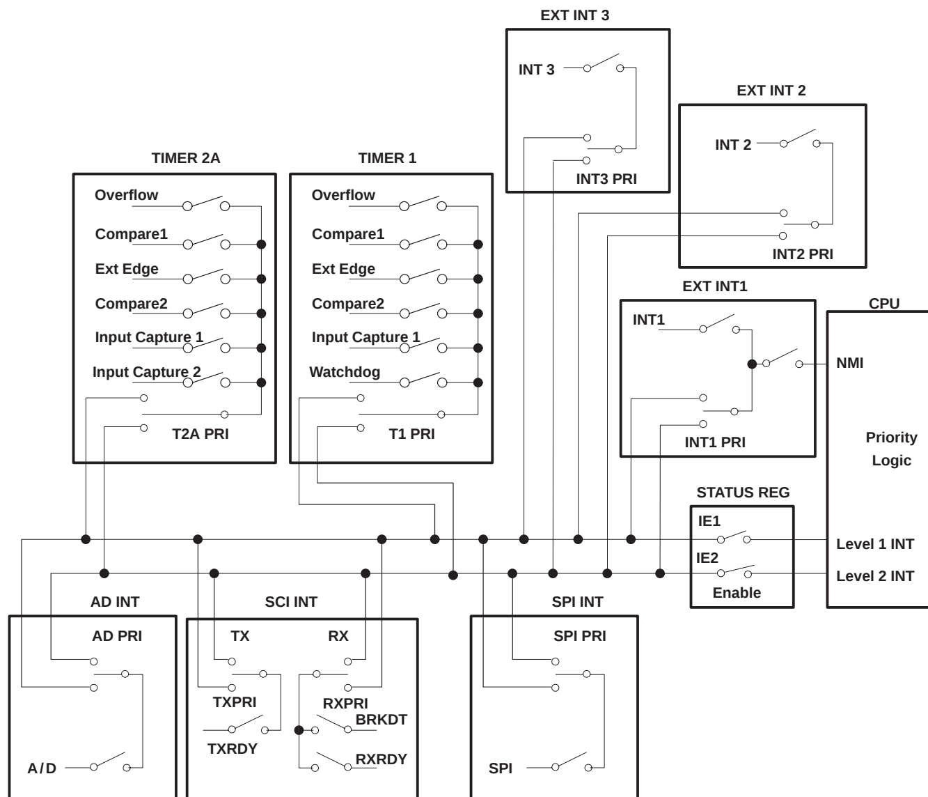
Figure 4. Interrupt Control
