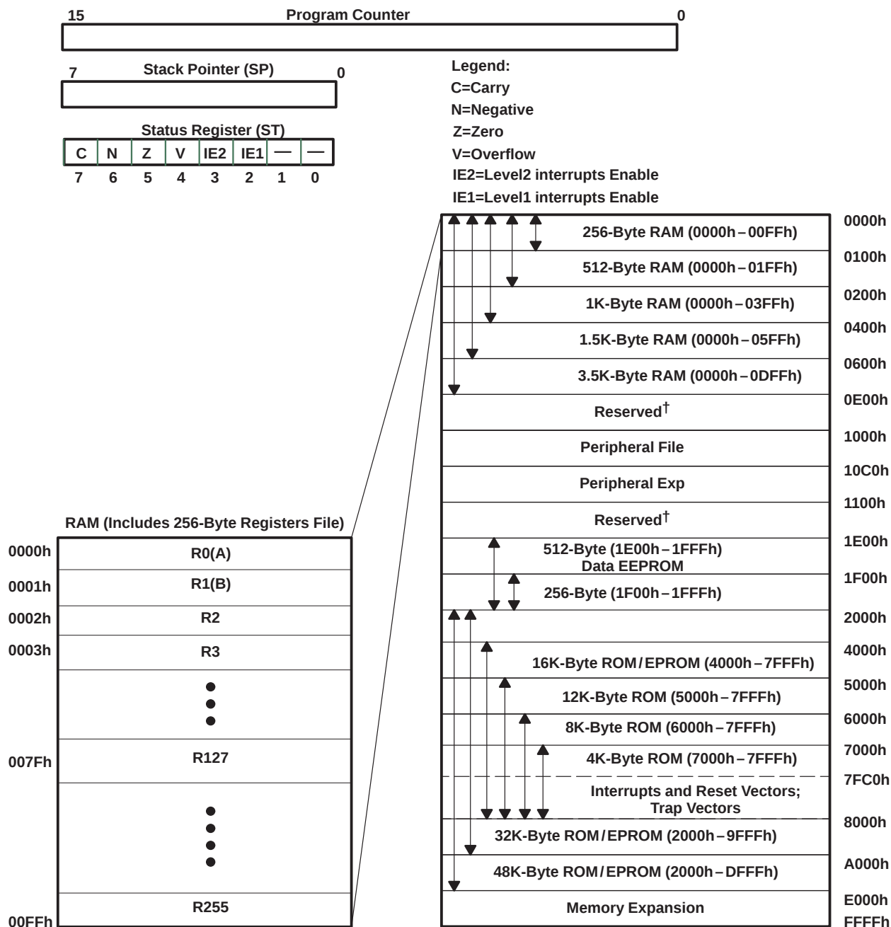
Figure 1. Programmer's Model
