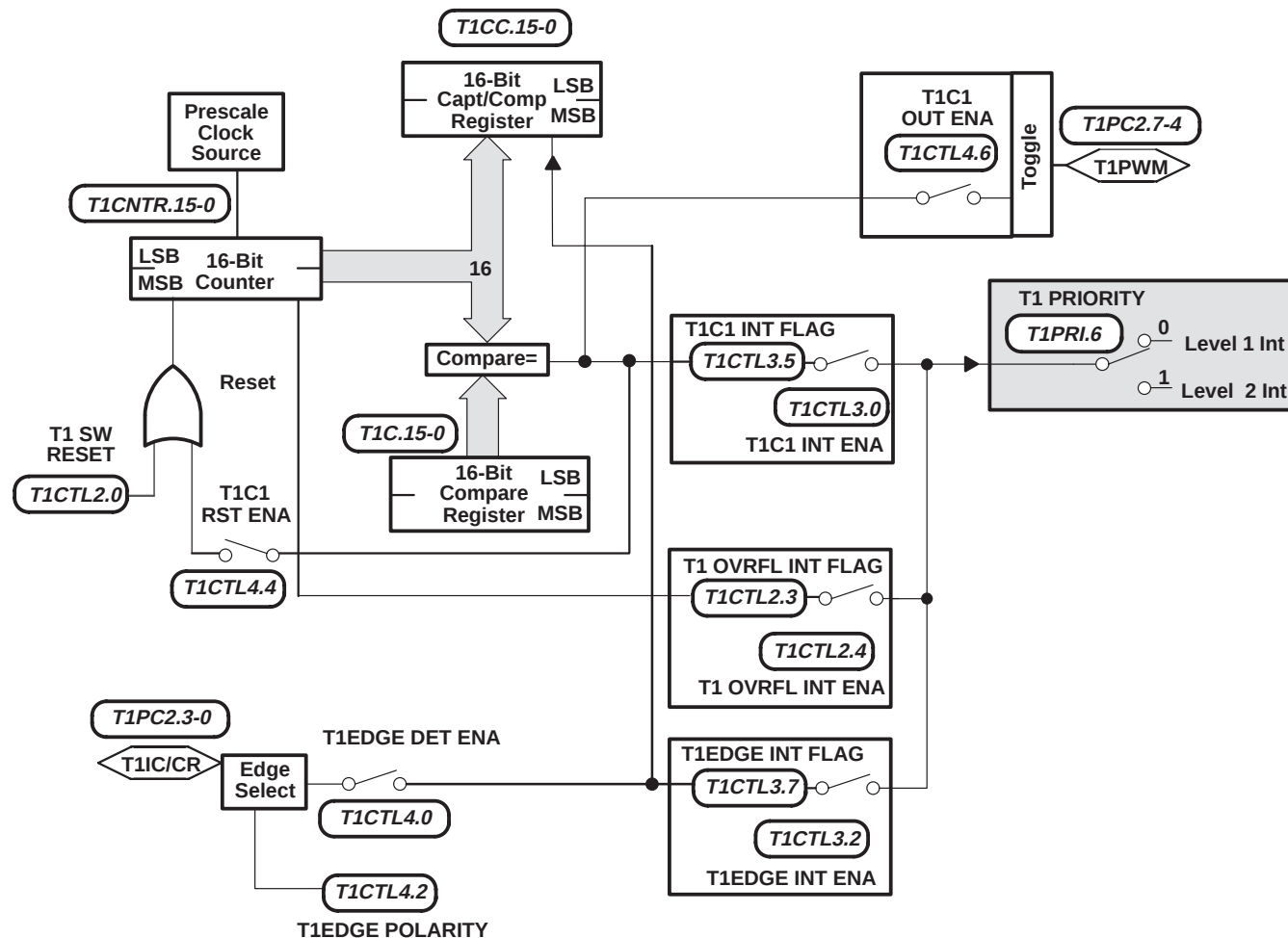
Figure 6. Capture/Compare Mode
