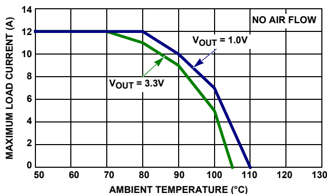
FIGURE 11. DERATING CURVE, 5V_{\text{IN}} , FOR VARIOUS OUTPUT VOLTAGES LISTED
