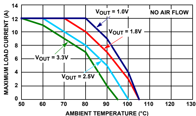
FIGURE 12. DERATING CURVE, 12V_{\text{IN}} , FOR VARIOUS OUTPUT VOLTAGES LISTED
