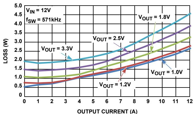
FIGURE 14. POWER LOSS CURVE, 12V_{\text{IN}} , FOR VARIOUS OUTPUT VOLTAGES LISTED
