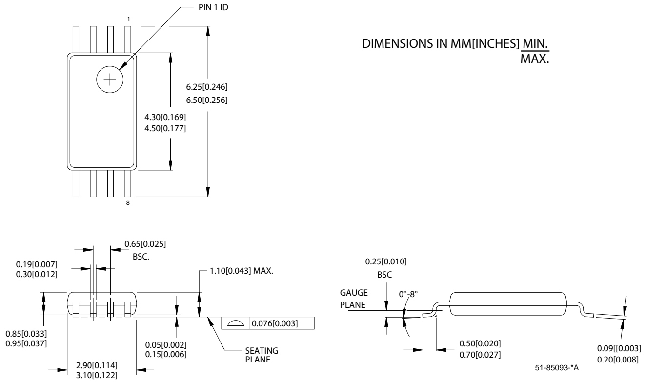
Figure 6. 8-Pin Thin Shrink Small Outline Package (4.40 MM Body) Z8 (51-85093)
