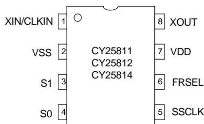
Figure 1. Pin Diagram - 8 Pin SOIC/TSSOP
