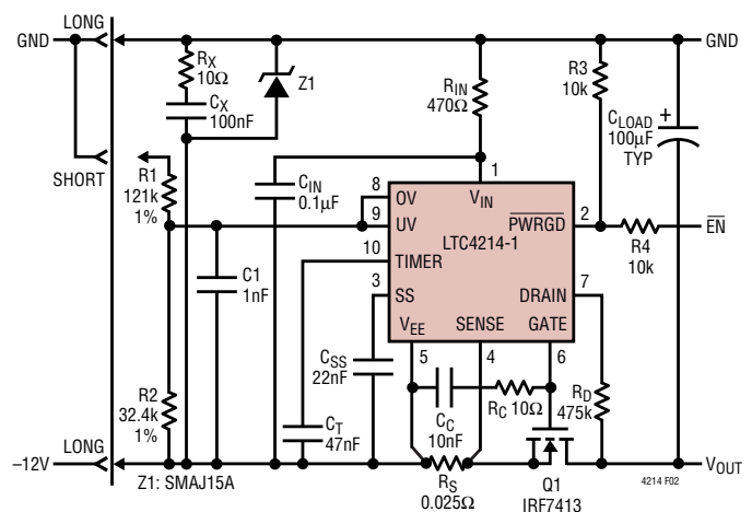
Figure 2. -12\text{V} , 2A Hot Swap Controller
