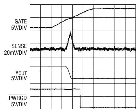
Start-Up Behavior
