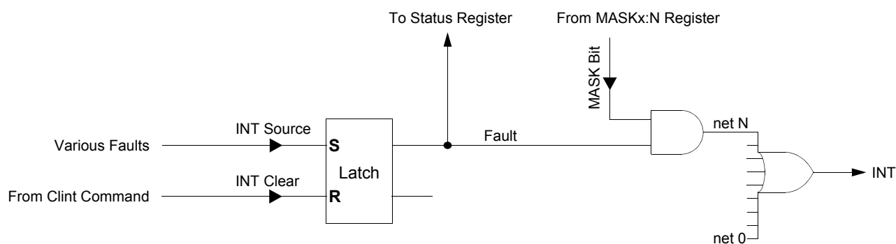
Figure 18. Interrupt Handling
