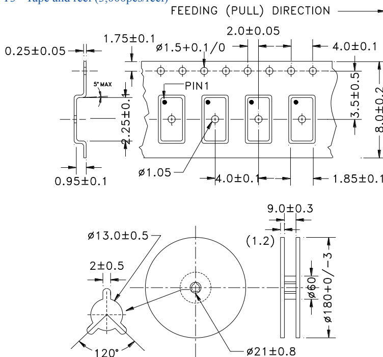
Dimensions: mm
