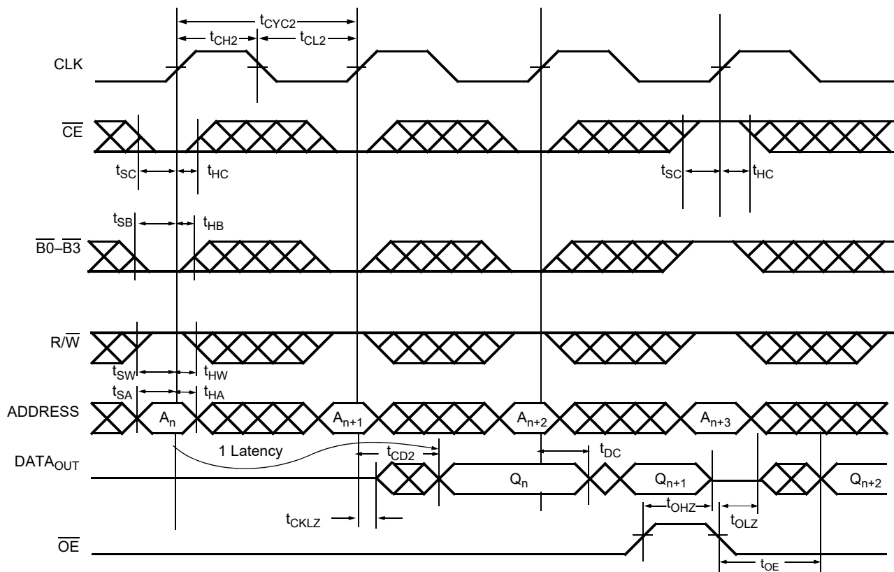
Figure 8. Read Cycle [32, 33, 34, 35, 36]
