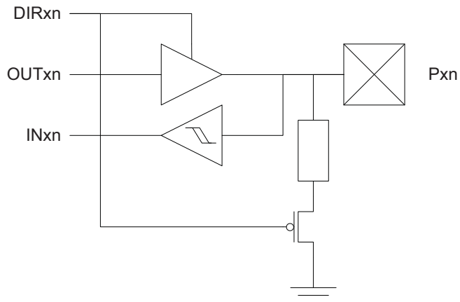
Figure 14-2. I/O Configuration - Totem-pole with Pull-down (on input)
