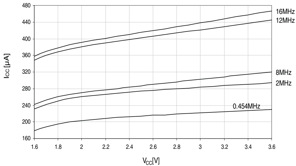
Figure 34-99. Standby Supply Current vs. V_{CC} 25°C, running from different crystal oscillators
