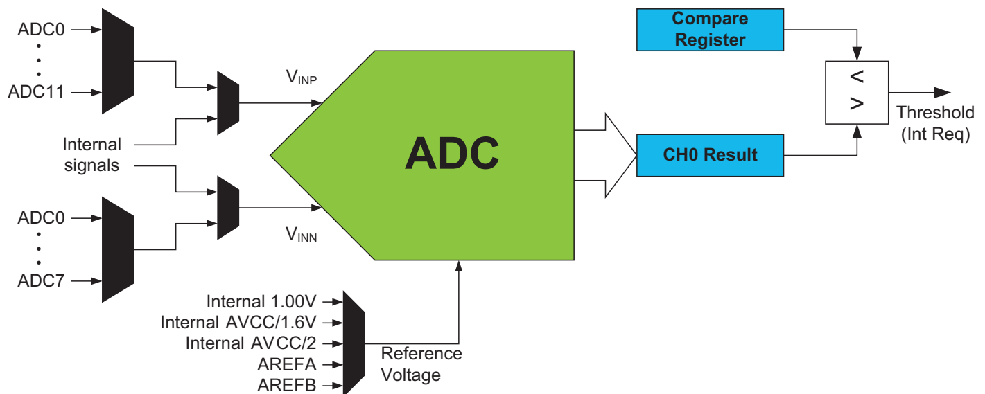
Figure 26-1. ADC Overview
