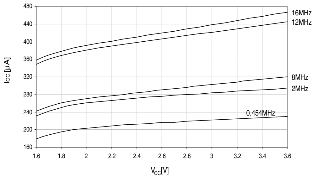
Figure 34-20. Standby Supply Current vs. V_{CC}
