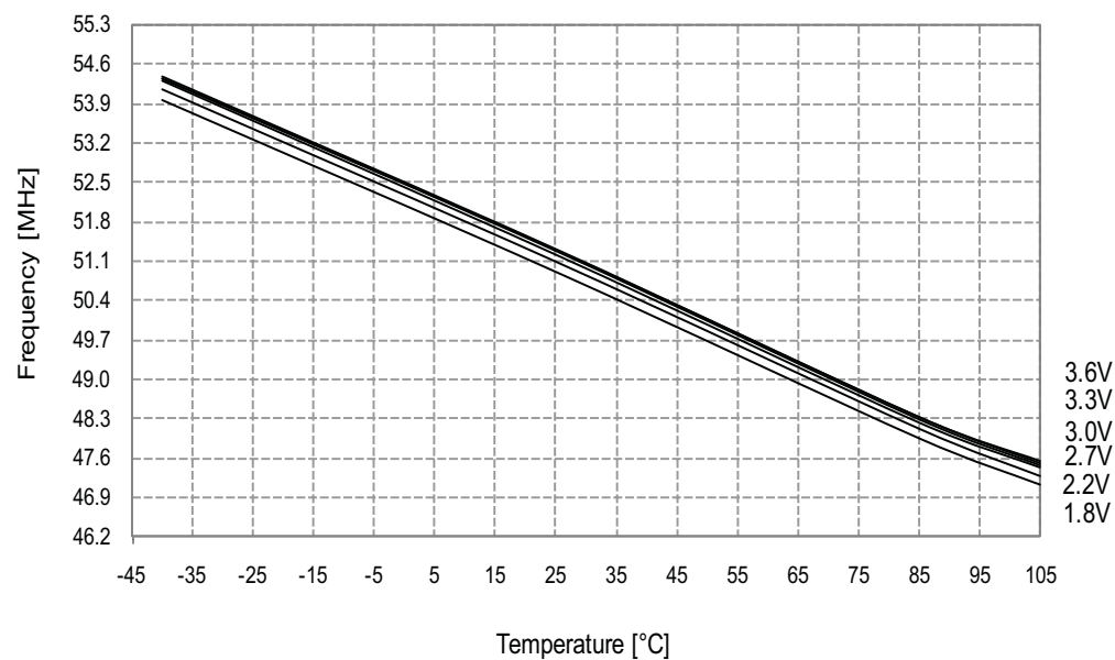
Figure 34-74. 48MHz Internal Oscillator Frequency vs. Temperature
