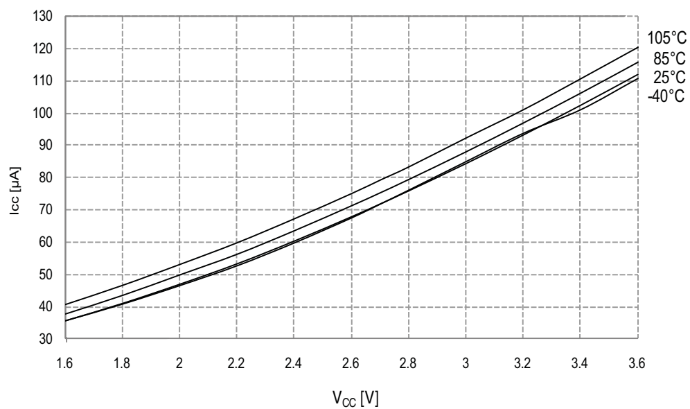
Figure 34-91. Idle Mode Supply Current vs. V_{CC}
