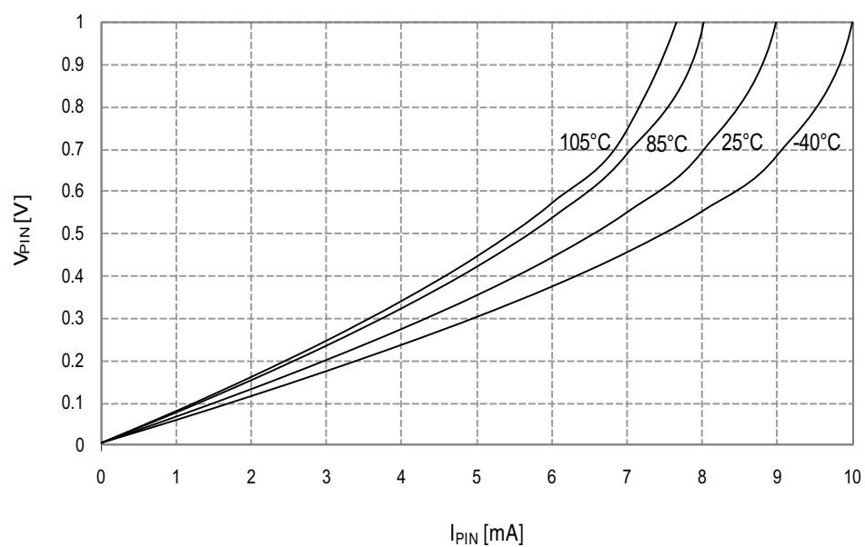
Figure 34-107. I/O Pin Output Voltage vs. Sink Current
