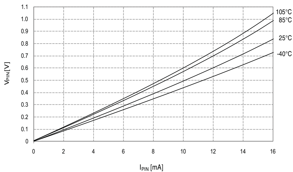
Figure 34-30. I/O Pin Output Voltage vs. Sink Current
