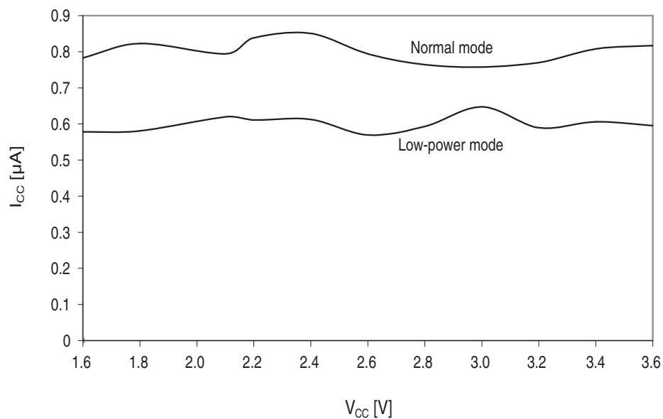
Figure 34-18. Power-save Mode Supply Current vs. V_{CC}
