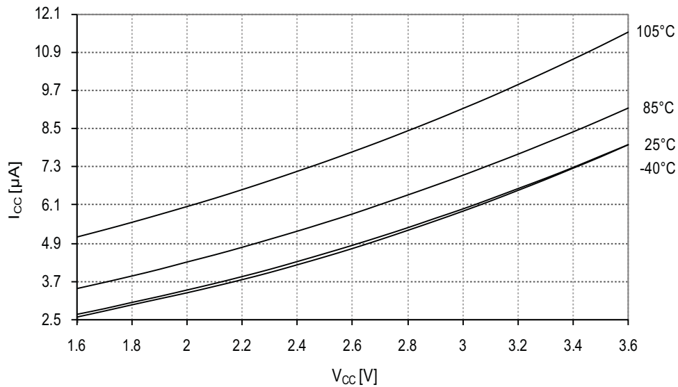
Figure 34-98. Standby Supply Current vs. V_{CC} Standby, f_{SYS} = 1\text{MHz}
