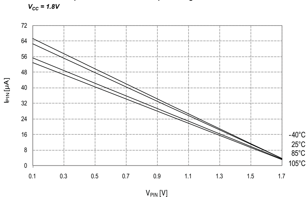
Figure 34-21. I/O Pin Pull-up Resistor Current vs. Input Voltage
