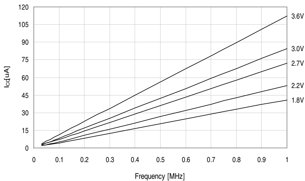
Figure 34-87. Idle Mode Supply Current vs. Frequency
