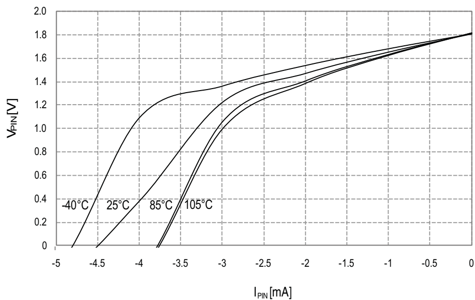
Figure 34-103. I/O Pin Output Voltage vs. Source Current
