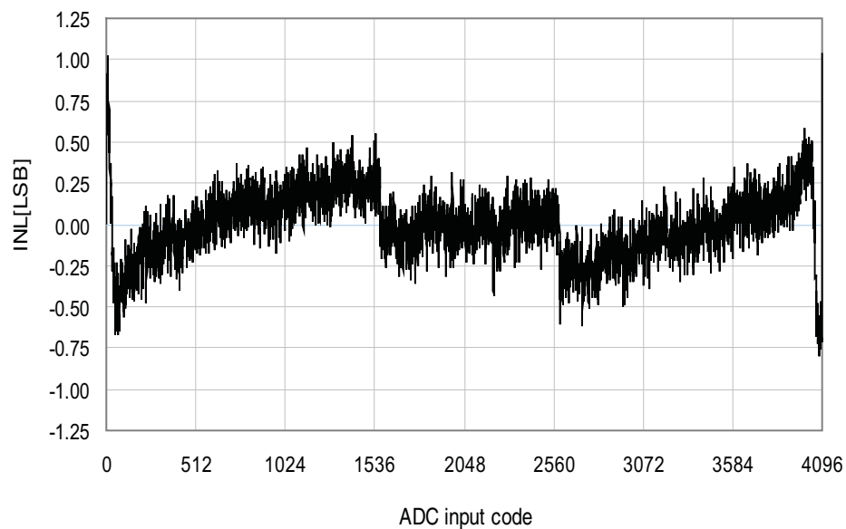
Figure 34-38. INL Error vs. Input Code
