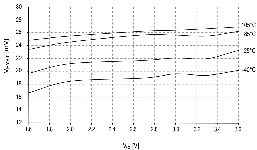
Figure 34-129. Analog Comparator Hysteresis vs. V_{CC} Low power, large hysteresis
