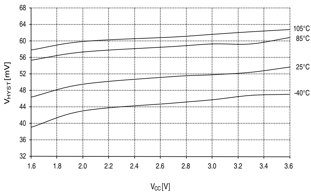
Figure 34-129. Analog Comparator Hysteresis vs. V_{CC} Low power, large hysteresis
