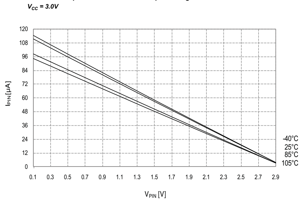
Figure 34-22. I/O Pin Pull-up Resistor Current vs. Input Voltage
