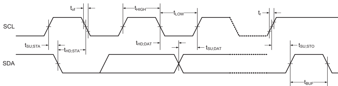
Figure 33-14. Two-wire Interface Bus Timing
