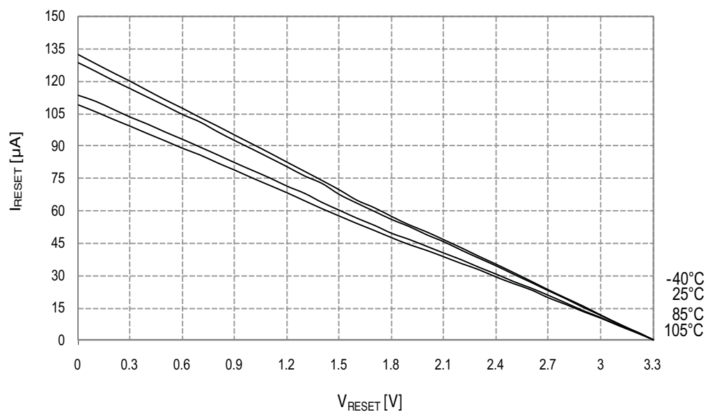
Figure 34-60. Reset Pin Pull-up Resistor Current vs. Reset Pin Voltage
