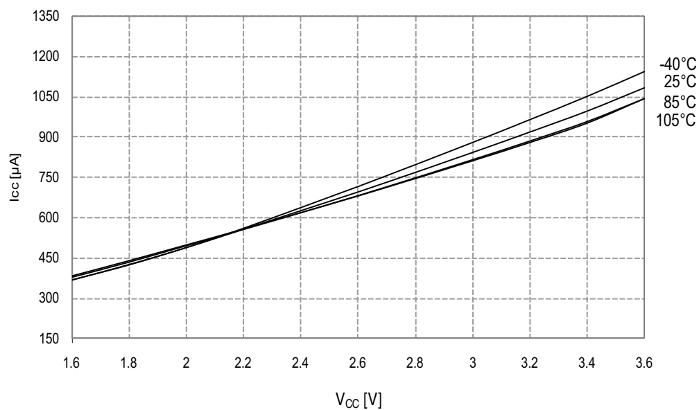
Figure 34-85. Active Mode Supply Current vs. V_{CC}
