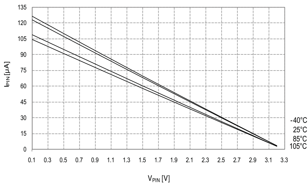
Figure 34-102. I/O Pin Pull-up Resistor Current vs. Input Voltage
