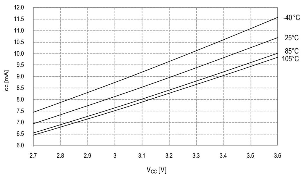
Figure 34-86. Active Mode Supply Current vs. V_{CC}
