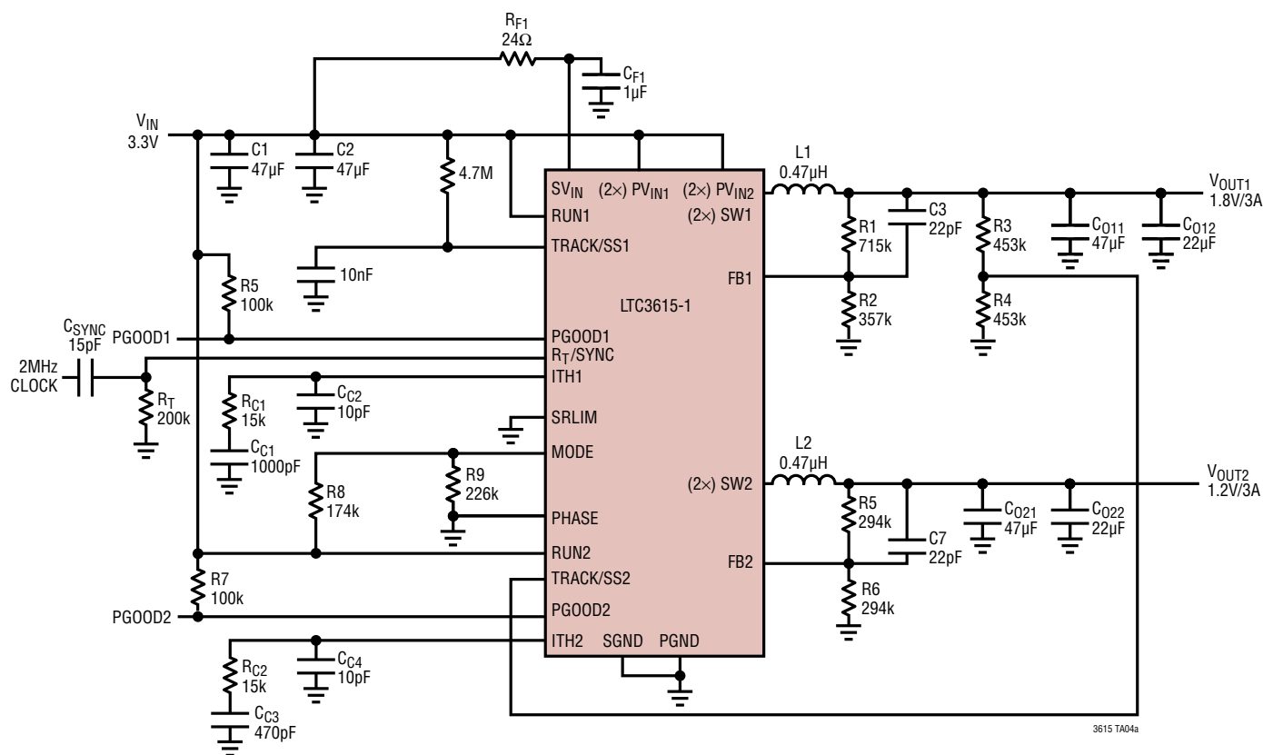
Master and Slave for Coincident Tracking Outputs Using a 2MHz External Clock
