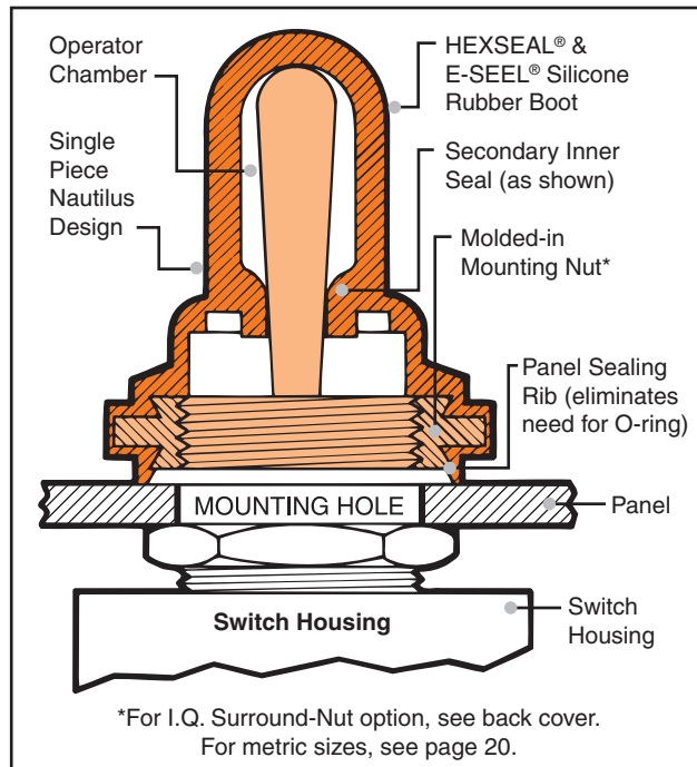
FIGURE 1 Full-Toggle Boot with Integral Secondary Inner Seal – IP66/68 Rated
