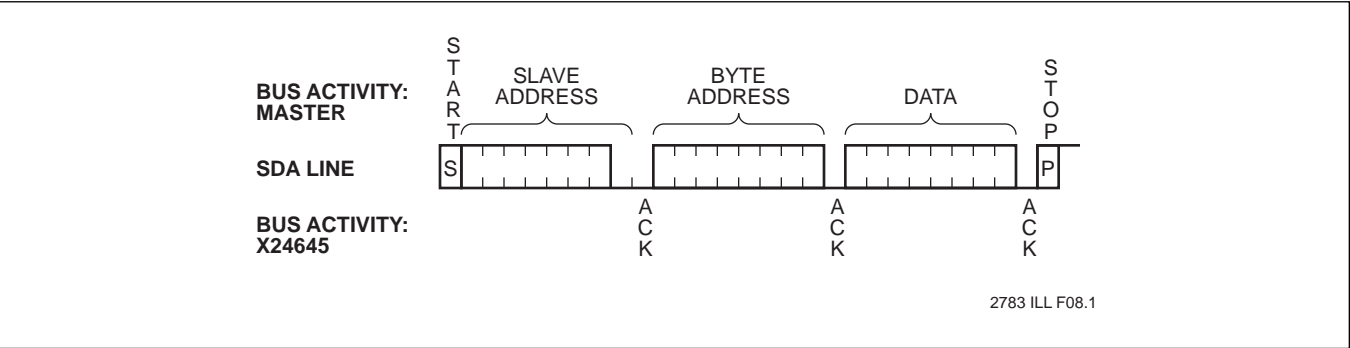
Figure 5. Byte Write
