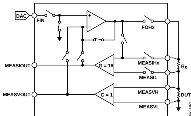
Figure 21. PMU in Standby Mode
