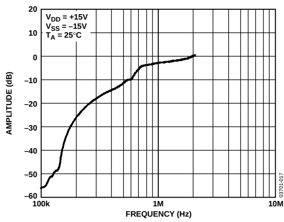
Figure 17. Voltage Sense Amplifier AC PSRR
