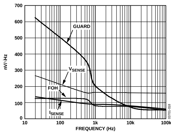
Figure 18. Noise Spectral Density
