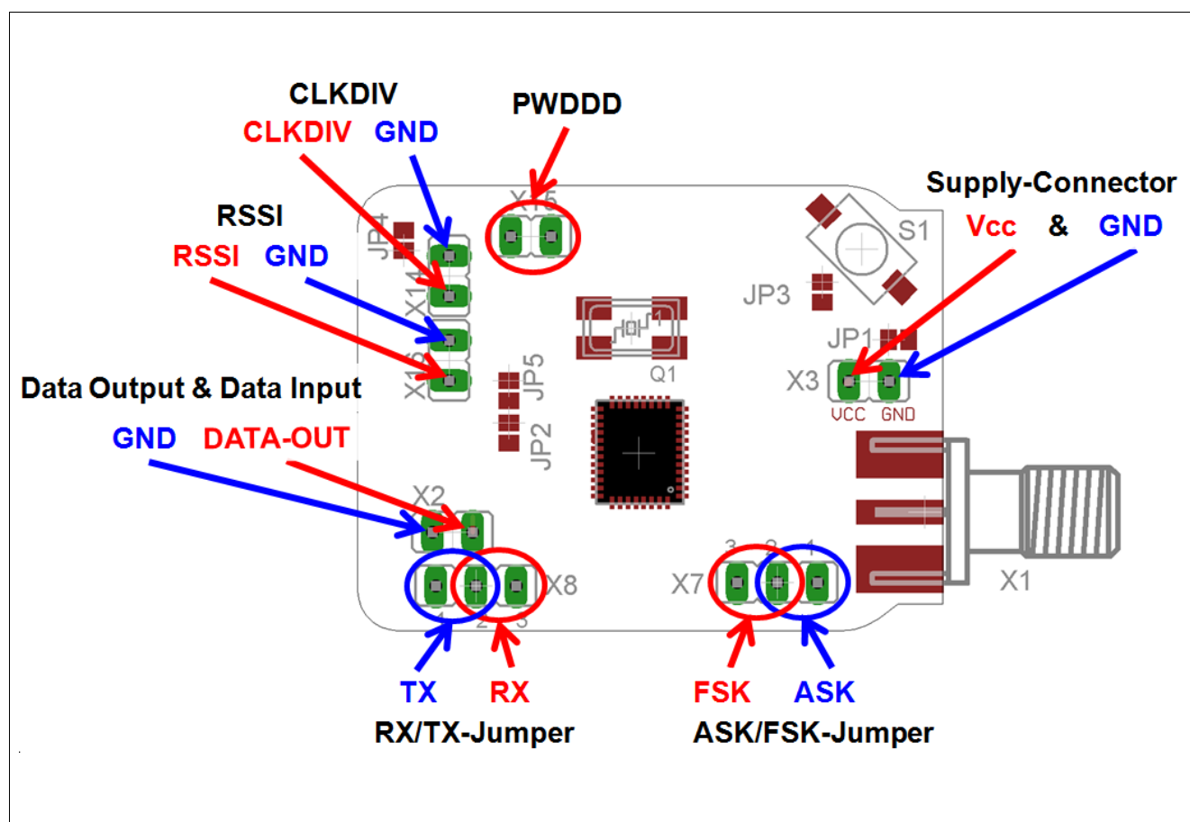
Figure 59 Placement of connectors and jumpers (axial)
