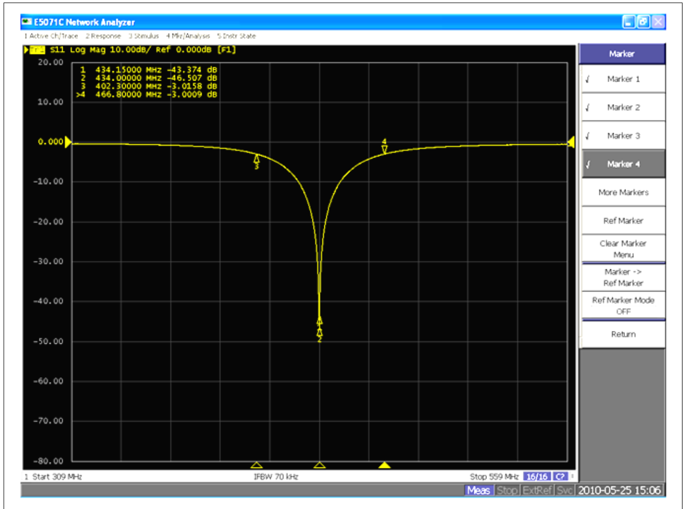
Figure 23 S11 Measured
