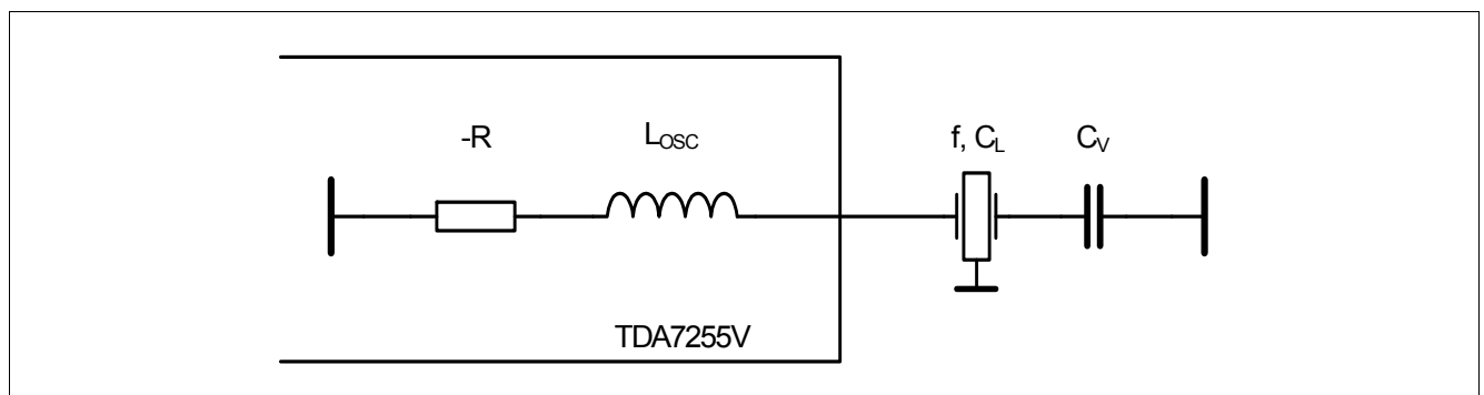
Figure 33 Crystal Oscillator
