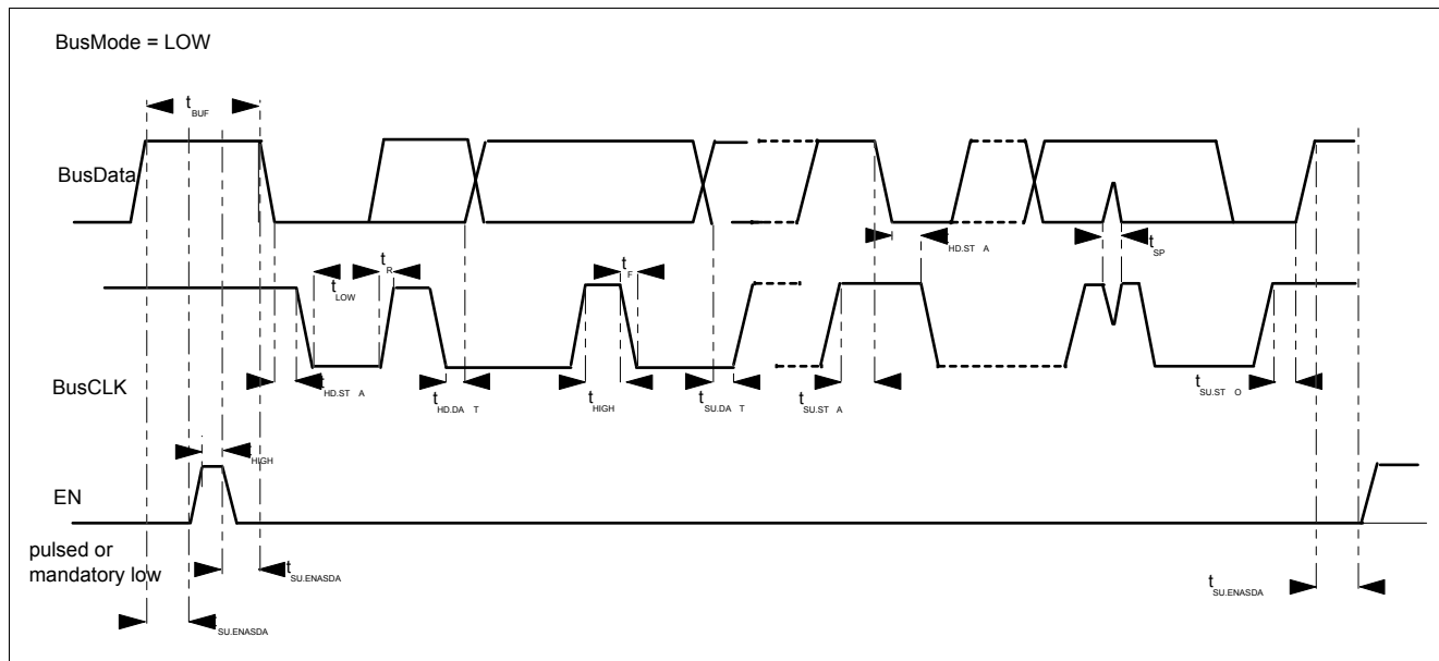
Figure 54 I 2 C Bus Timing
