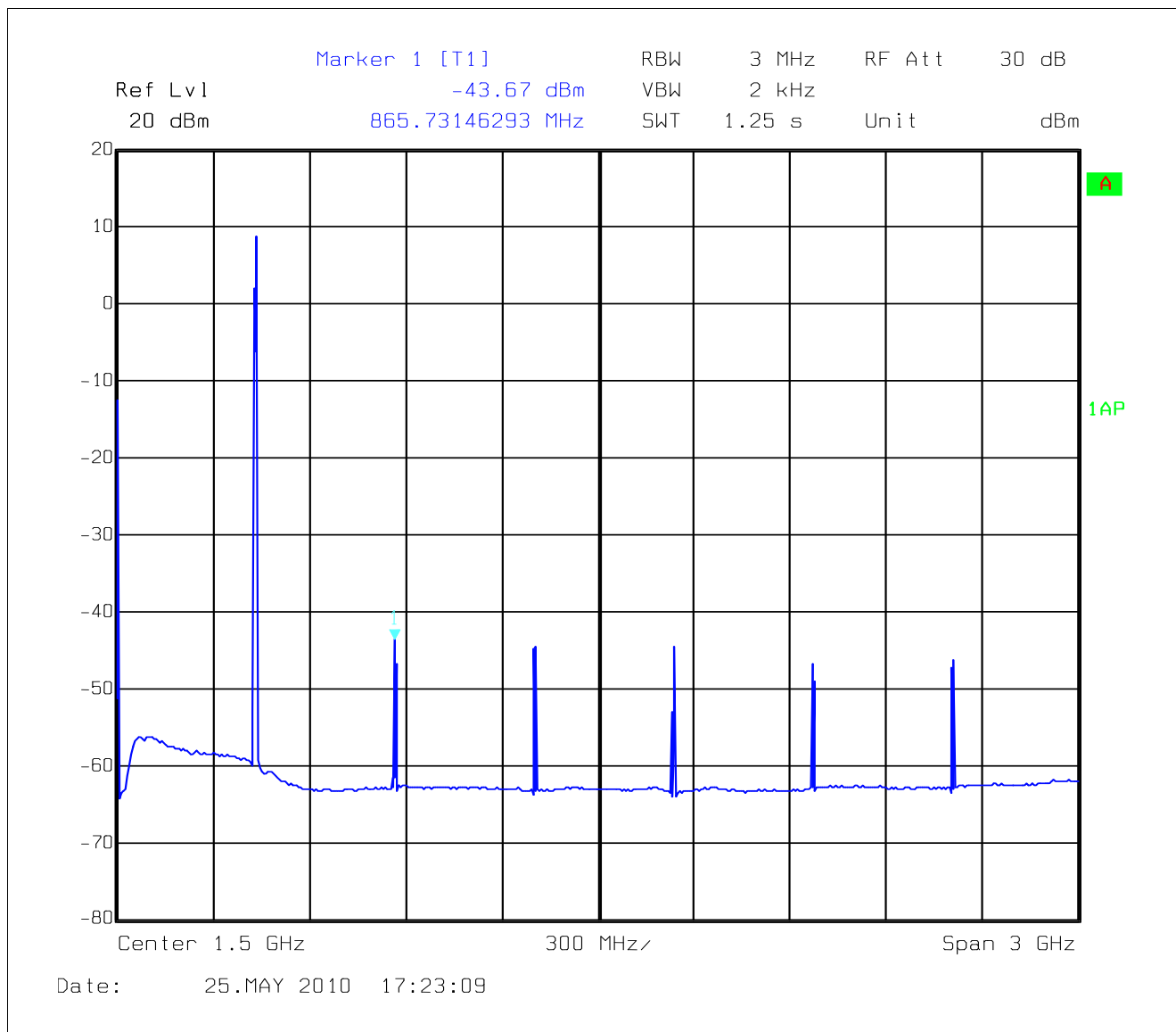
Figure 30 Transmit Spectrum 3 GHz
