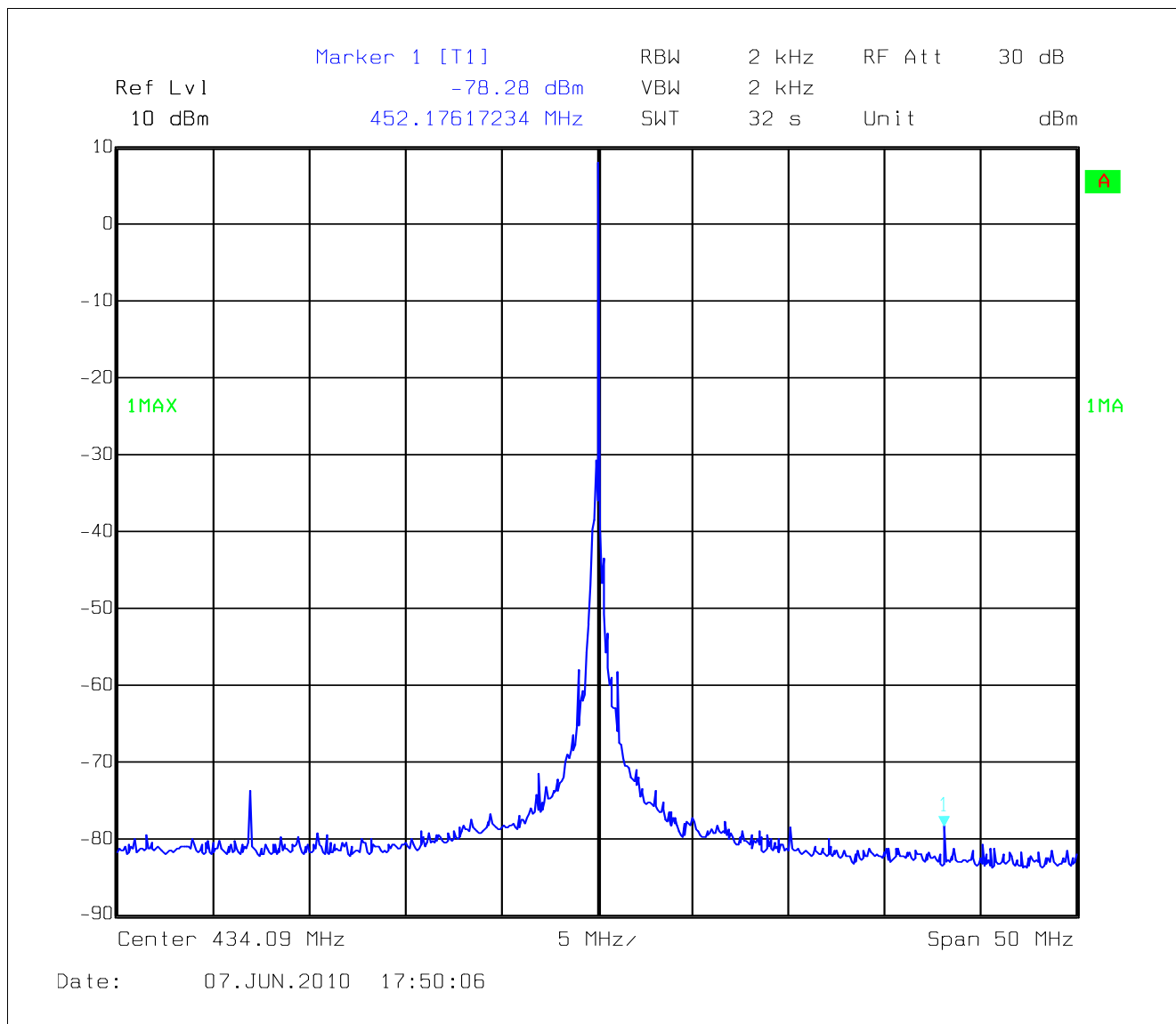
Figure 31 Transmit Spectrum X-tal-Oscillator Spurs
