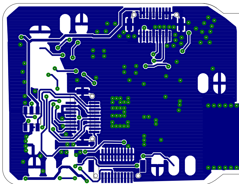
Figure 58 Bottom Layer of the Customer Board TDA7255V
