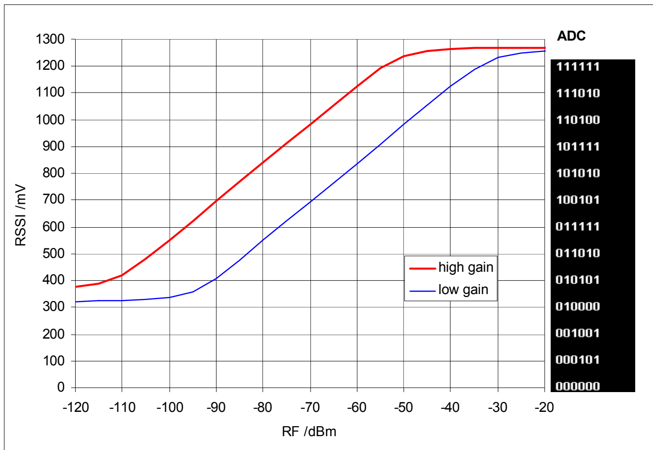
Figure 42 Typ. RSSI Level (Eval Board) @ 3 V
