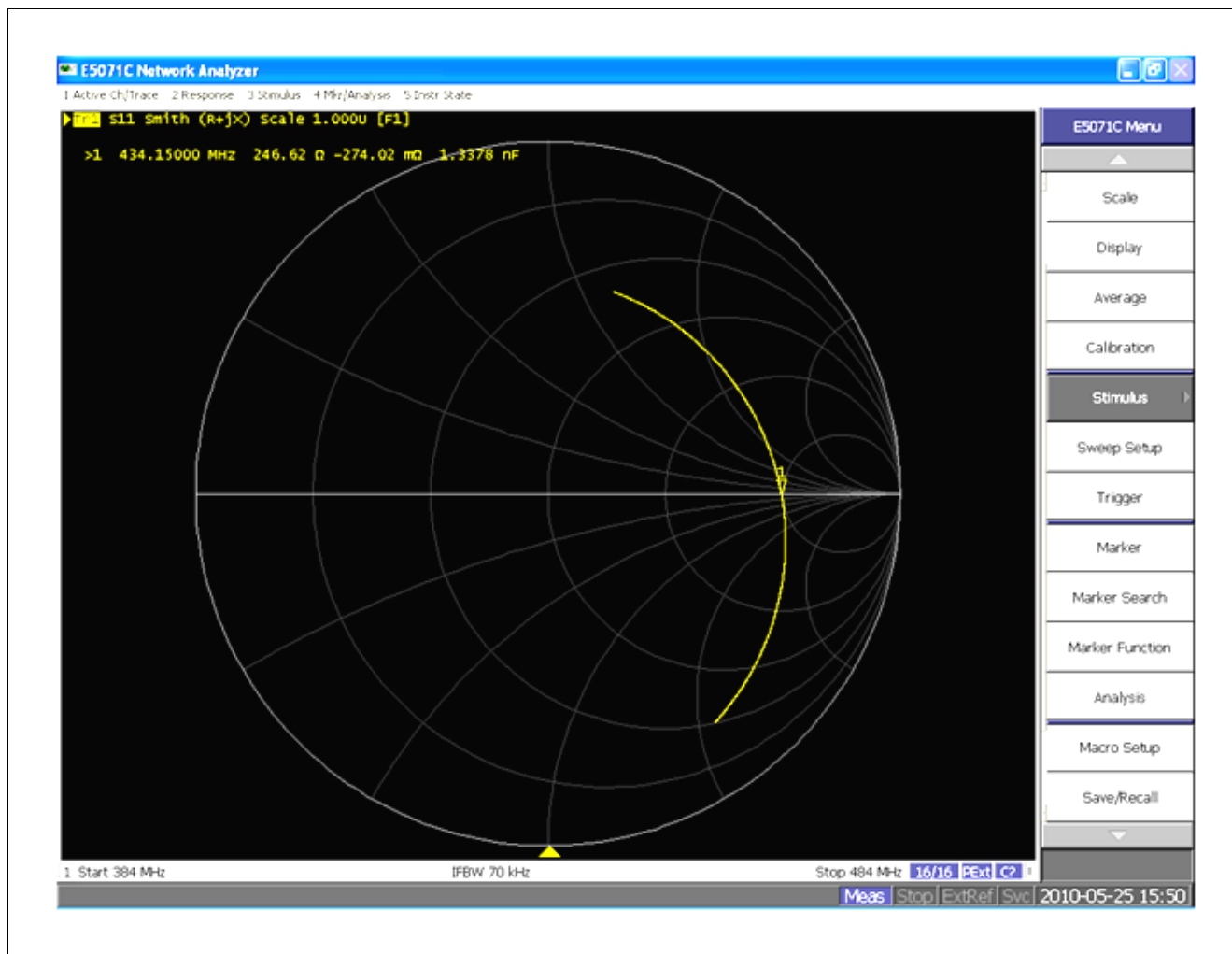
Figure 29 S11-Parameter measured 100 MHz
