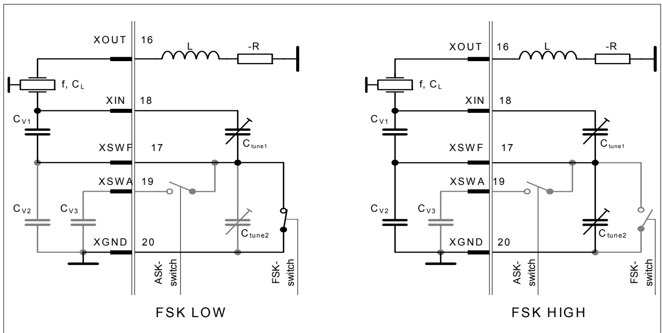
Figure 35 FSK Modulation
