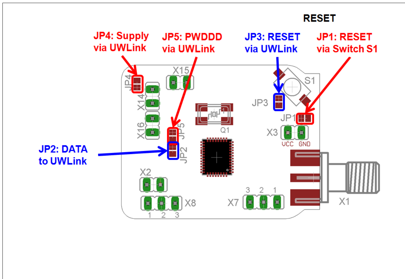
Figure 60 Placement of connectors and jumpers (SMD)
