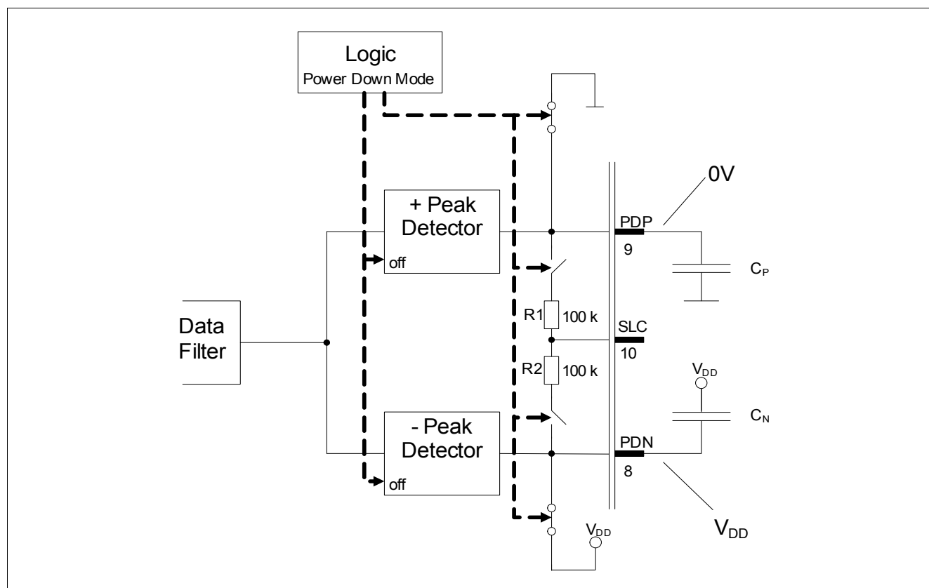
Figure 47 Peak Detector - Power Down Mode
