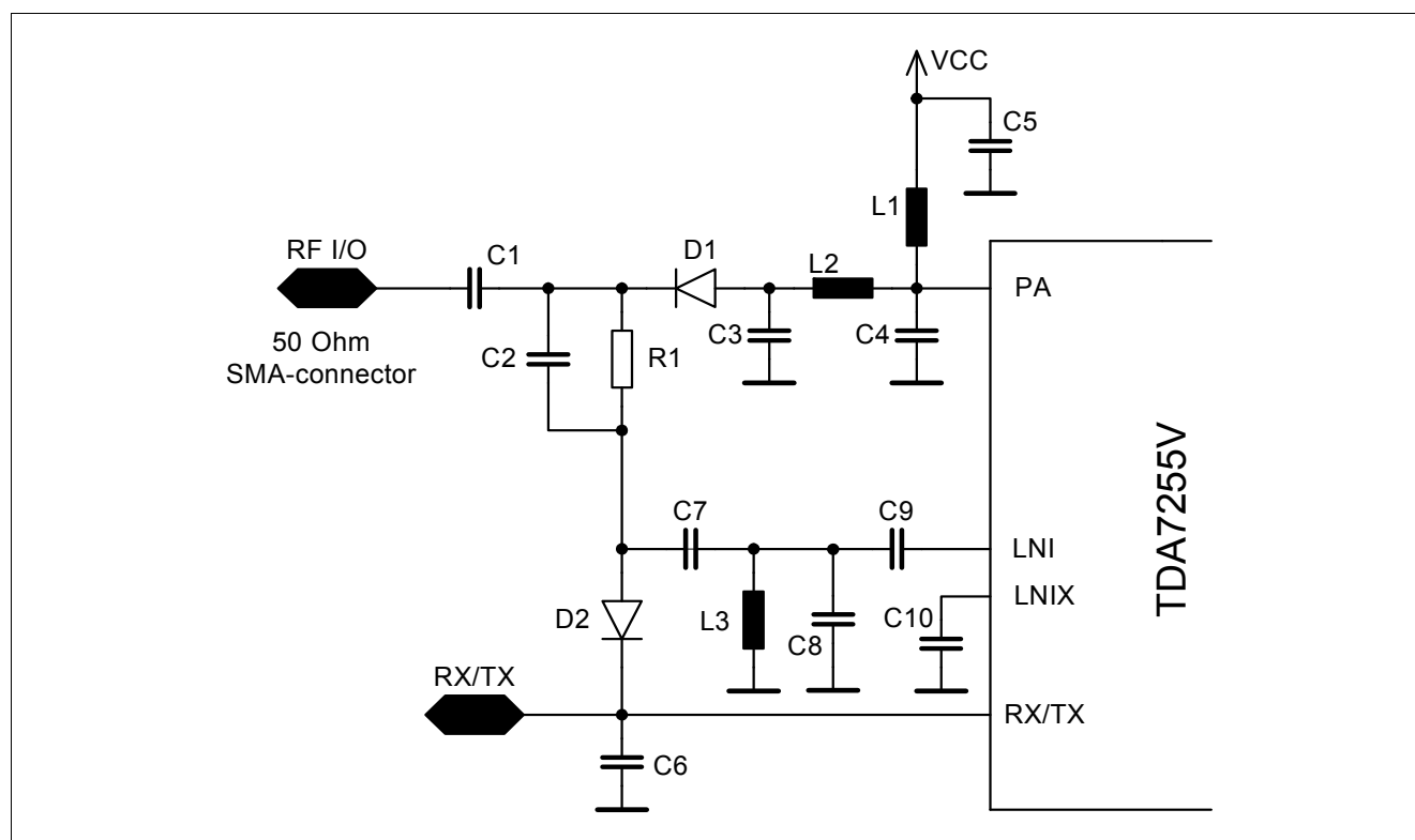
Figure 21 RX/TX-Switch
