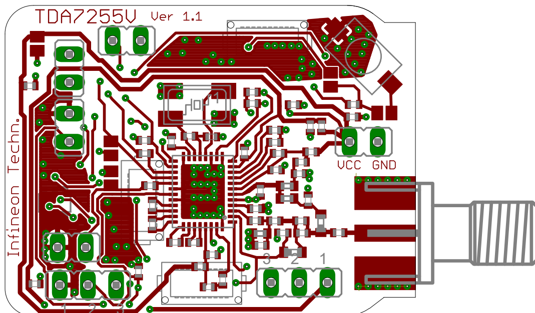
Figure 57 Top Layer of the Customer Board TDA7255V
