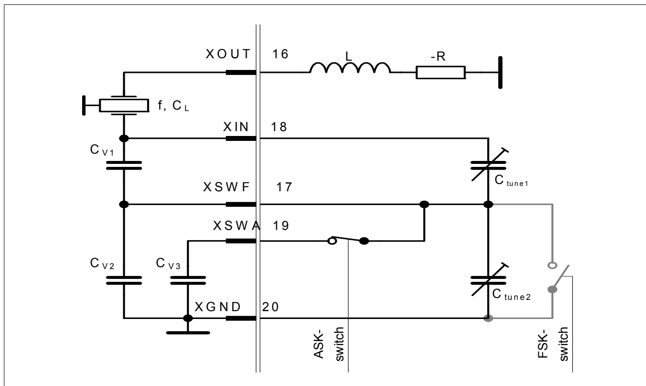
Figure 36 FSK Receive
