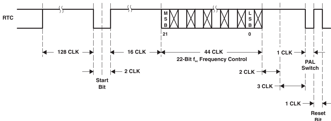
Figure 3-10. RTC Timing
