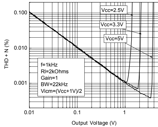
Figure 15. Distortion + noise vs. output voltage
