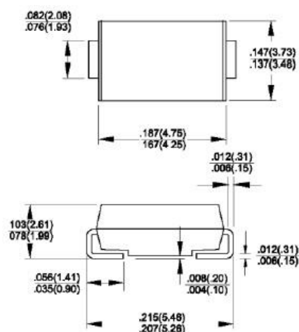
DO-214AA (SMB)
