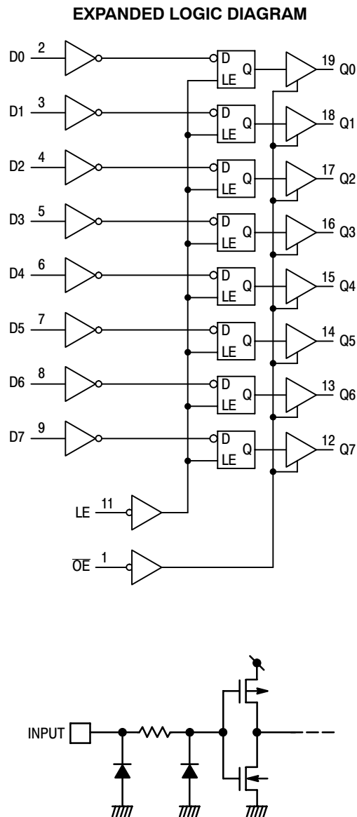
Figure 7. Input Equivalent Circuit
