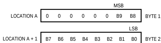
DO UT from LTC1091 Stored in MC68HC05C4 RAM
