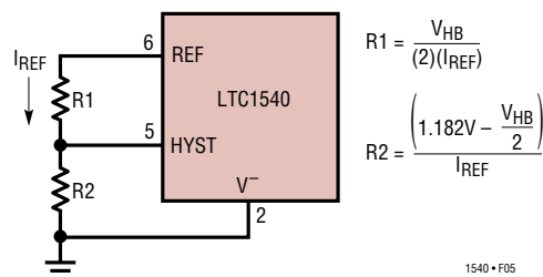
Figure 5. Programmable Hysteresis
