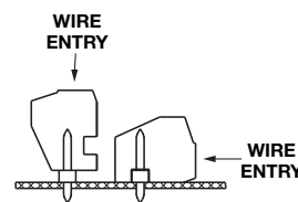
Mating orientations
