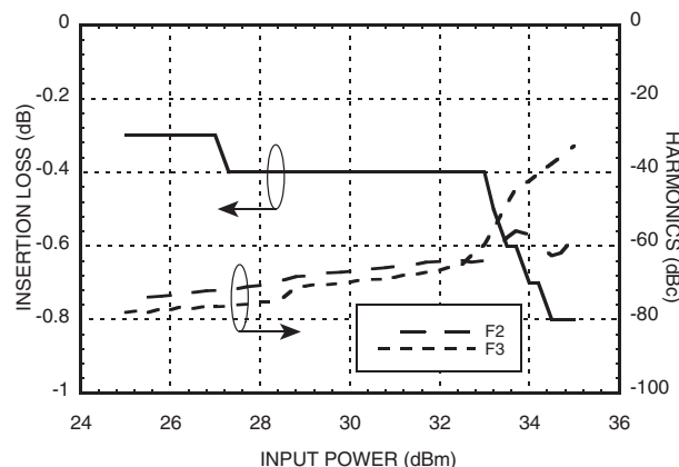
2nd & 3rd Harmonics @ 900 MHz Vdd = +3 Volts
