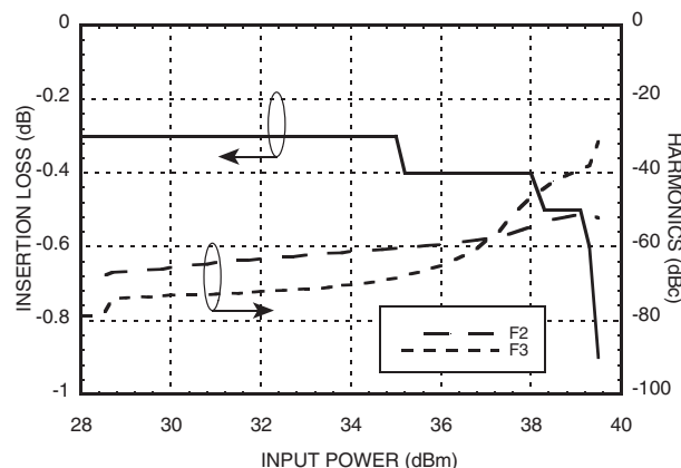
2nd & 3rd Harmonics @ 900 MHz Vdd = +8 Volts
