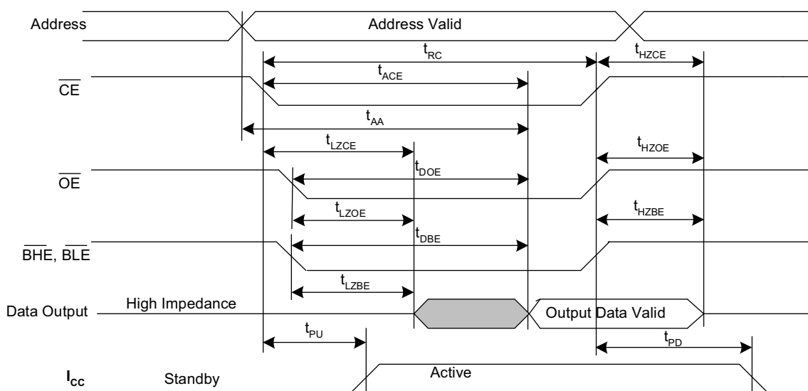
Figure 9. SRAM Read Cycle No. 2 ( \overline{\text{CE}} and \overline{\text{OE}} Controlled) [32, 34, 35]
