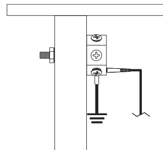
Figure 11. Mounting the 09837 Multi Ground Hub to a table leg.
