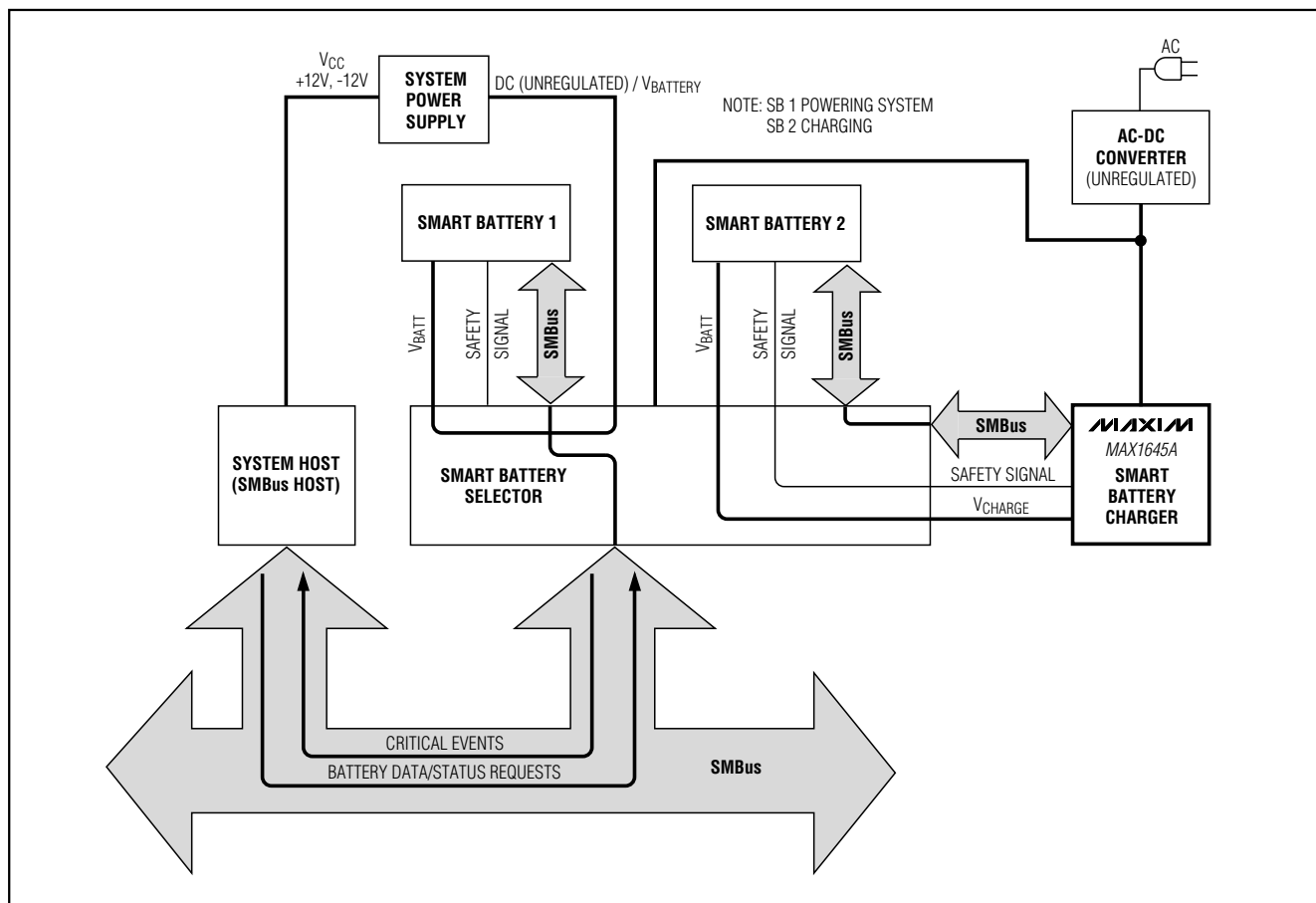
Figure 11. Typical System Using Multiple Smart Batteries
