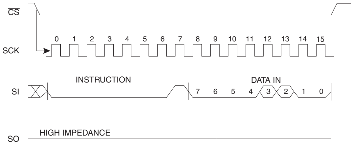
Figure 6-5. WRSR Timing
