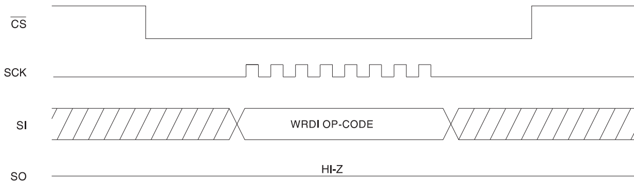
Figure 6-3. WRDI Timing
