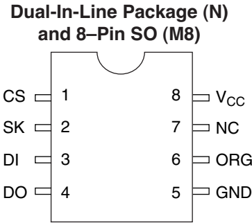
Top View Package Number N08E and M08A
