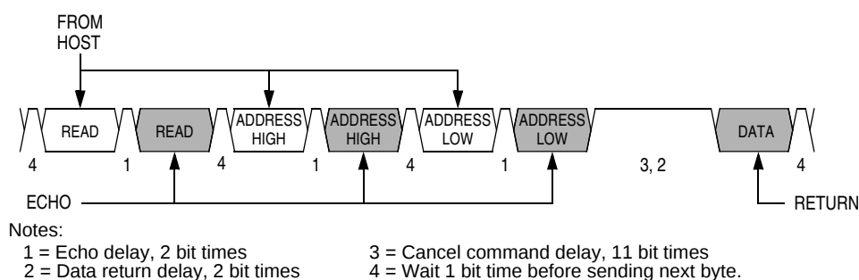
Figure 15-16. Read Transaction
