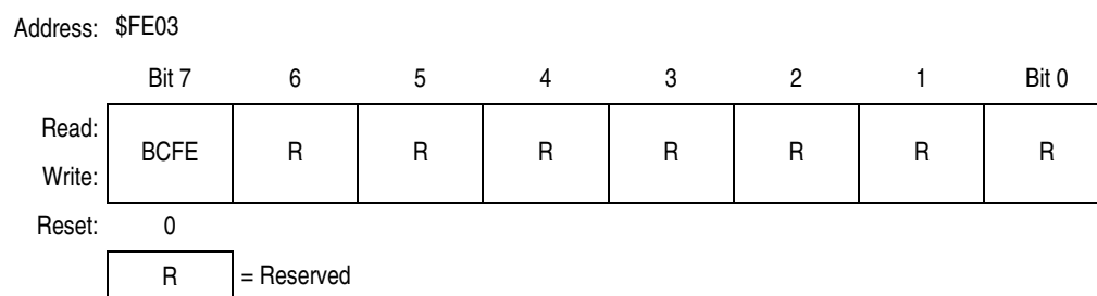
Figure 15-9. Break Flag Control Register (BFCR)
