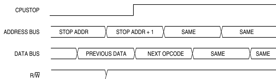
Figure 13-18. Stop Mode Entry Timing
