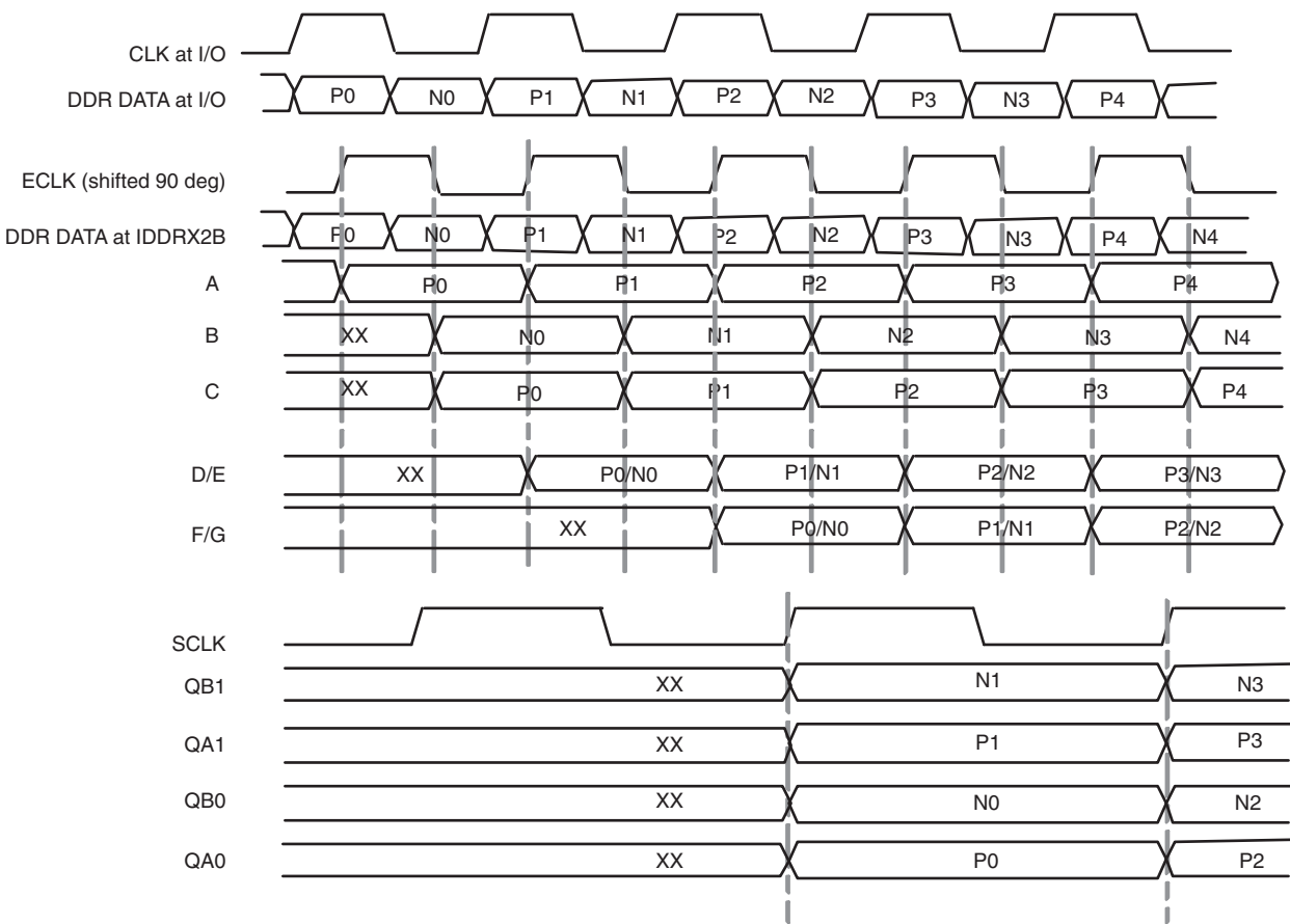
Figure 12-34. IDDRX2B Waveform
