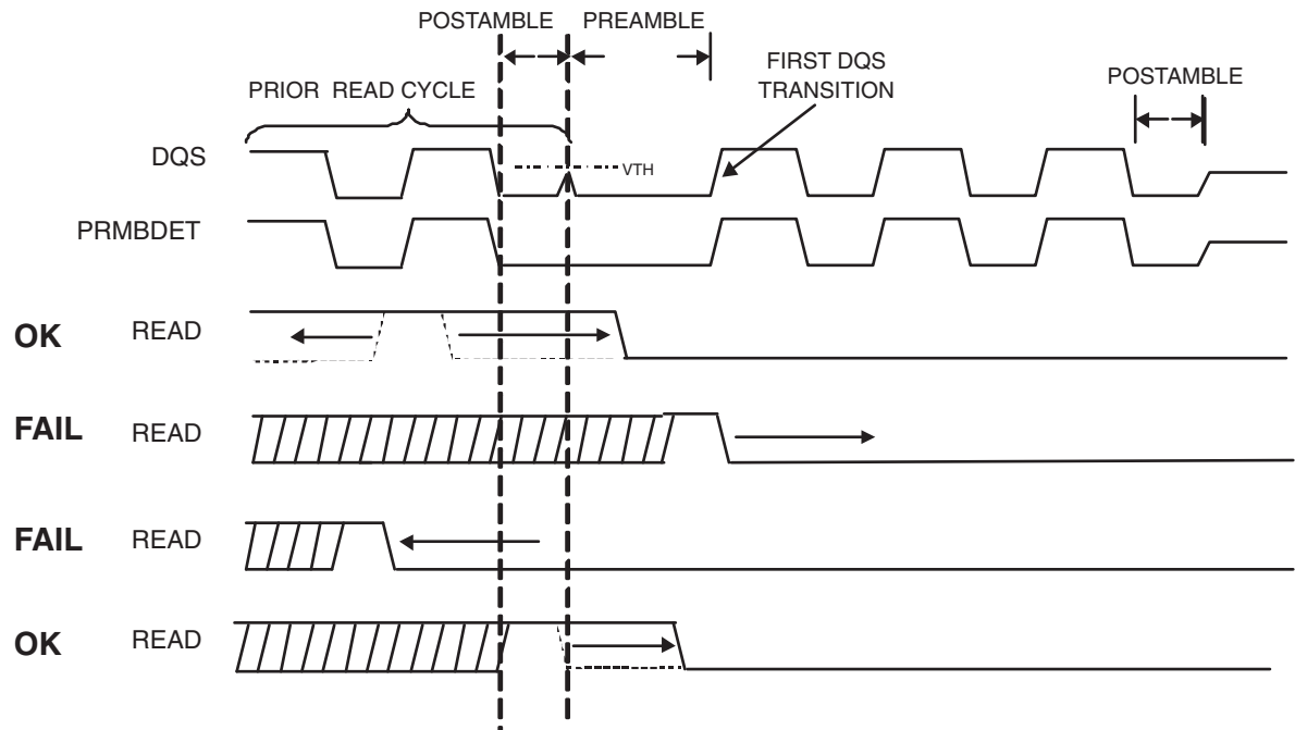
Figure 12-9. READ Pulse Generation
