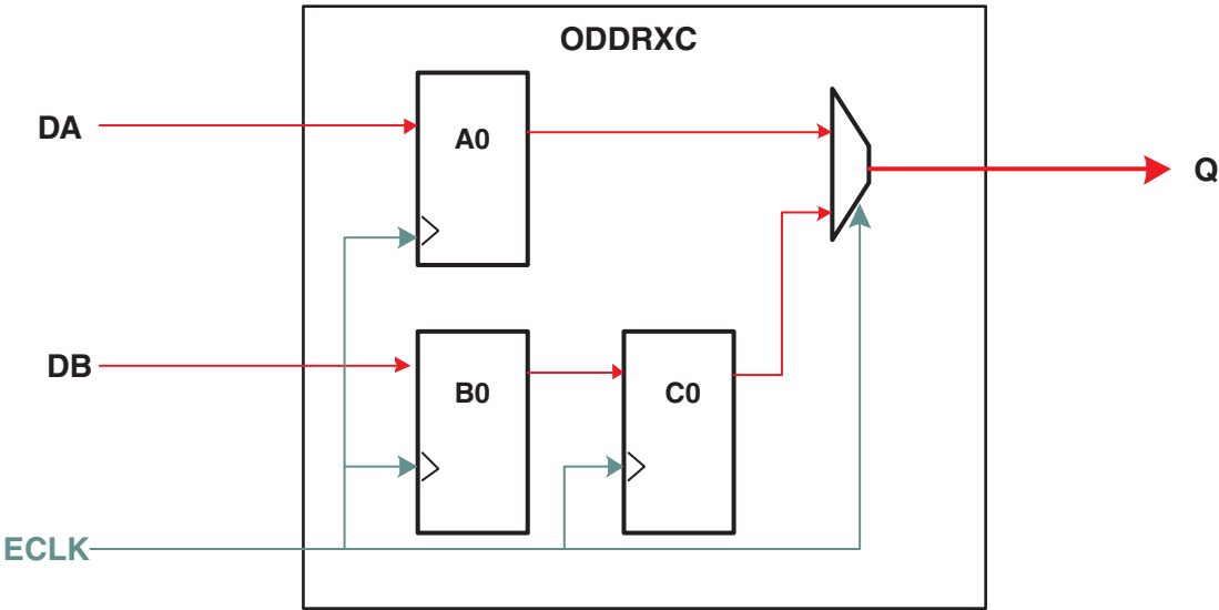
Figure 12-36. Output Register Block in ODDRXC Mode
