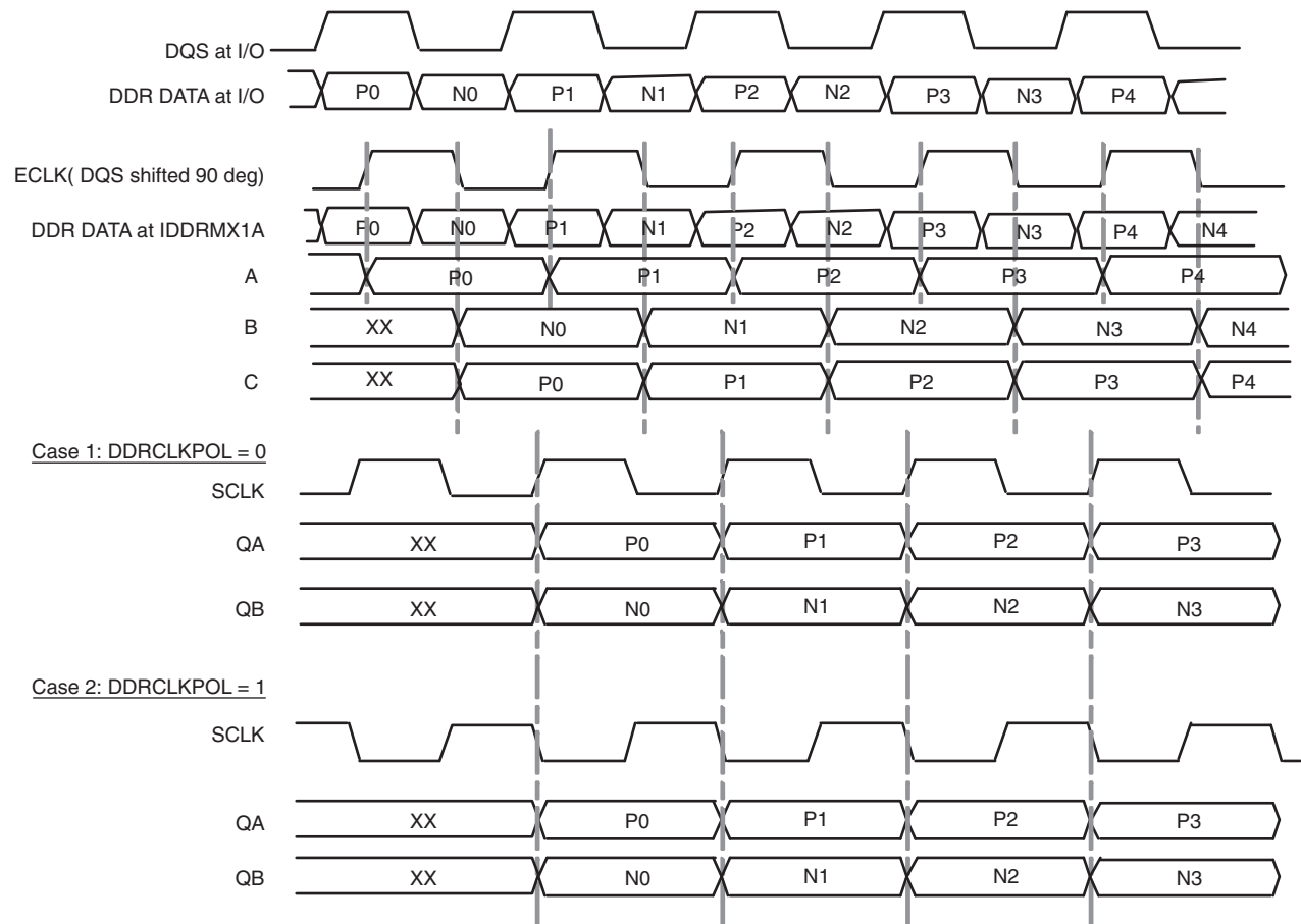
Figure 12-12. IDDRMX1A Waveform
