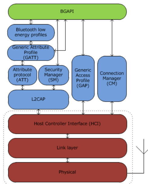
Figure 1: Bluetooth 4.0 single mode stack
