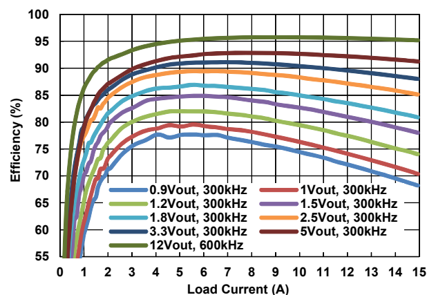
Figure 11. V_{IN} = 30\text{V}
