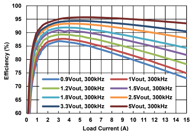
Figure 9. V_{IN} = 12\text{V}
