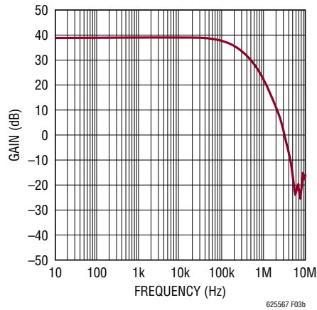
Figure 3. Gain of 100 Amplifier (3dB Bandwidth of 200kHz on 130μA Supply Current)
