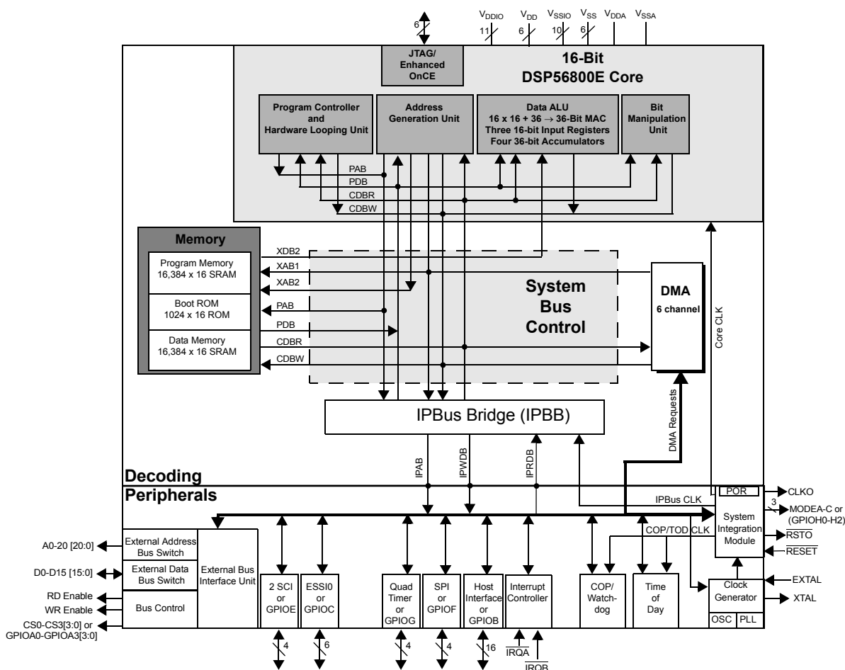
56854 Block Diagram
