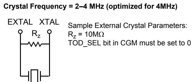
Figure 4-6 Crystal Oscillator
