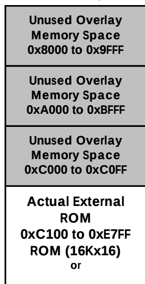
Bit 12 (ROM Merge) of the Extended Memory Controller Register = 0
