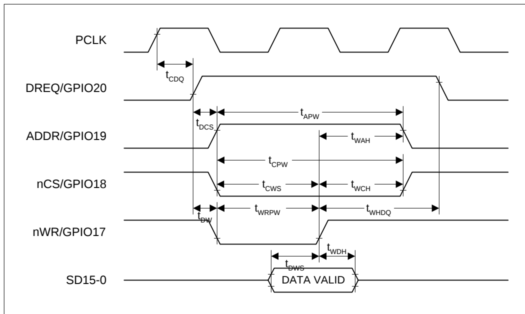
Figure 3-4. Mailbox/DMA Write
