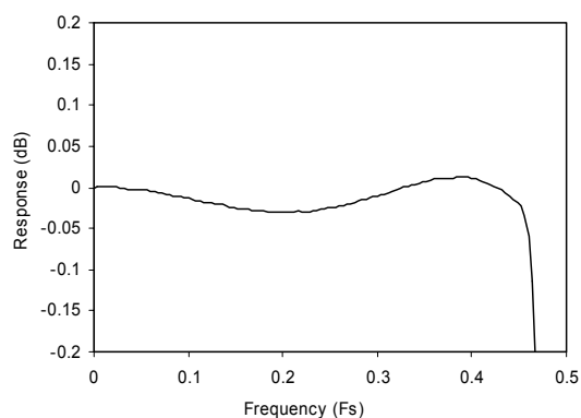
Figure 37 DAC Digital Filter Ripple
