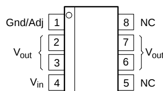
SO-8 D SUFFIX CASE 751
