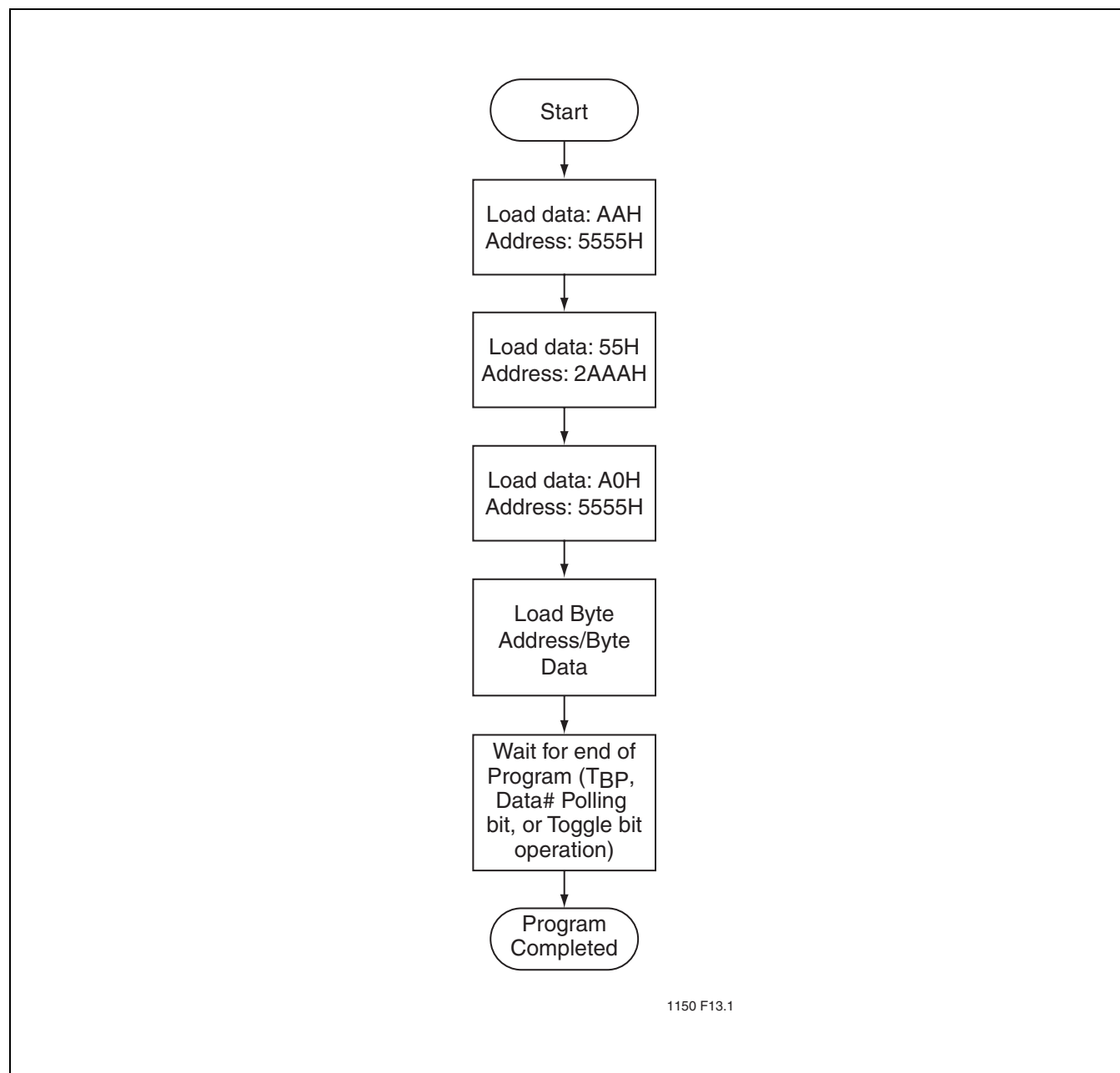
FIGURE 17: Byte-Program Algorithm
