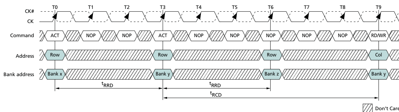
Figure 43: Example: Meeting t_{\text{RRD}}(\text{MIN}) and t_{\text{RCD}}(\text{MIN})
