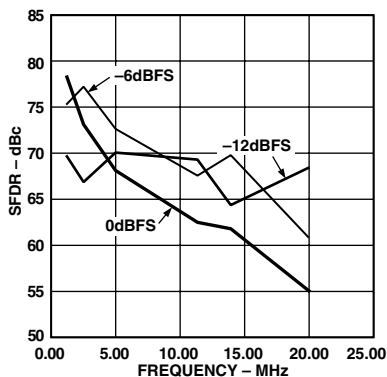
Figure 6. SFDR vs. f_{OUT} @ 50 MSPS
