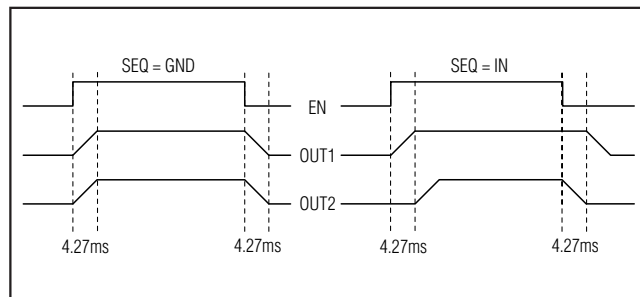
Figure 3. Timing Diagram
