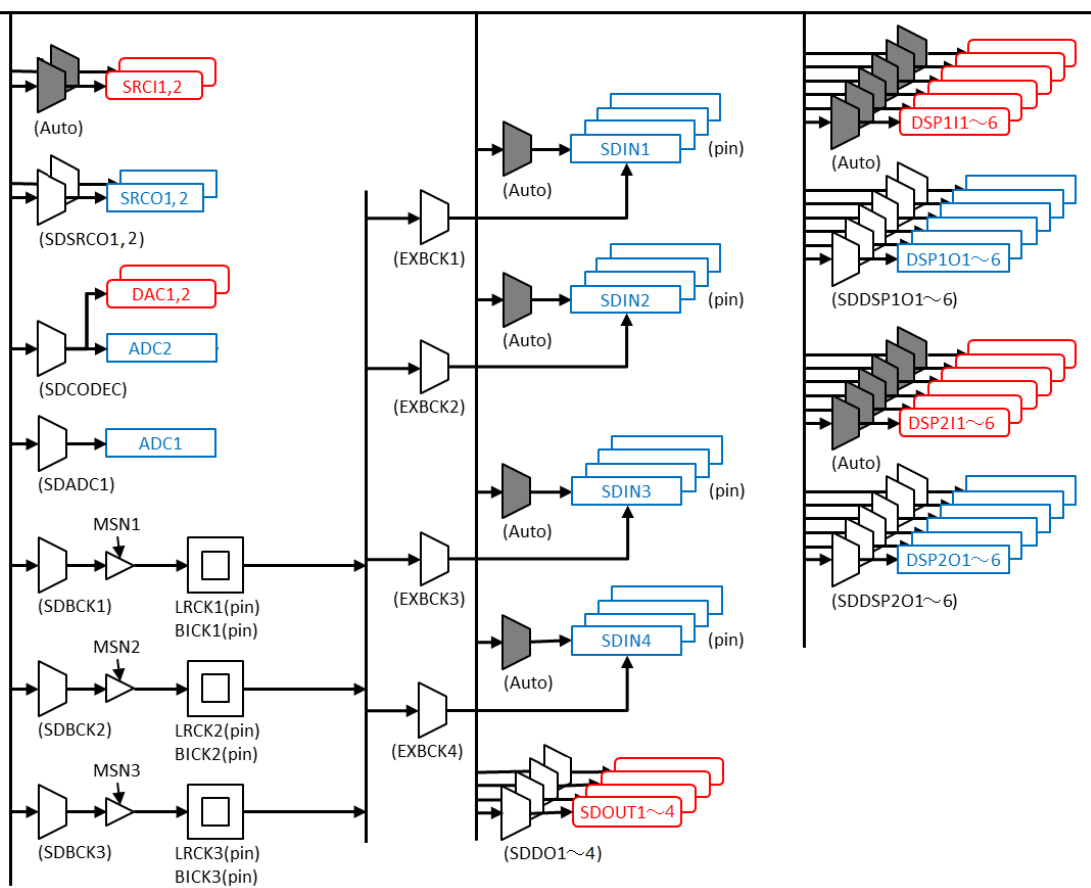
Figure 20. Clock Sync Domain Setting
