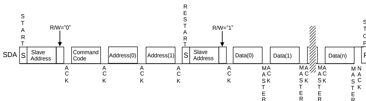
Figure 68. Read Sequence (I 2 C)
