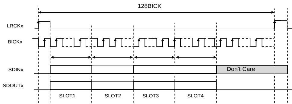
Figure 41. TDM Mode PCM Short Frame (BICK=128fs, BCKP bit = "0") * 57
