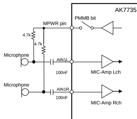
Figure 72. MIC Block Circuit (Single-end Input)
