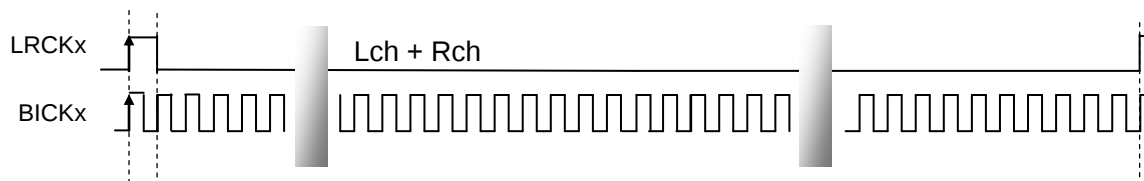
Figure 24. PCM Short Frame / PCM Long Frame (BCKPx bit = "1")
