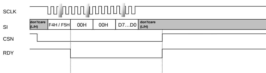
Figure 60. External Conditional Jump Timing (SPI)
