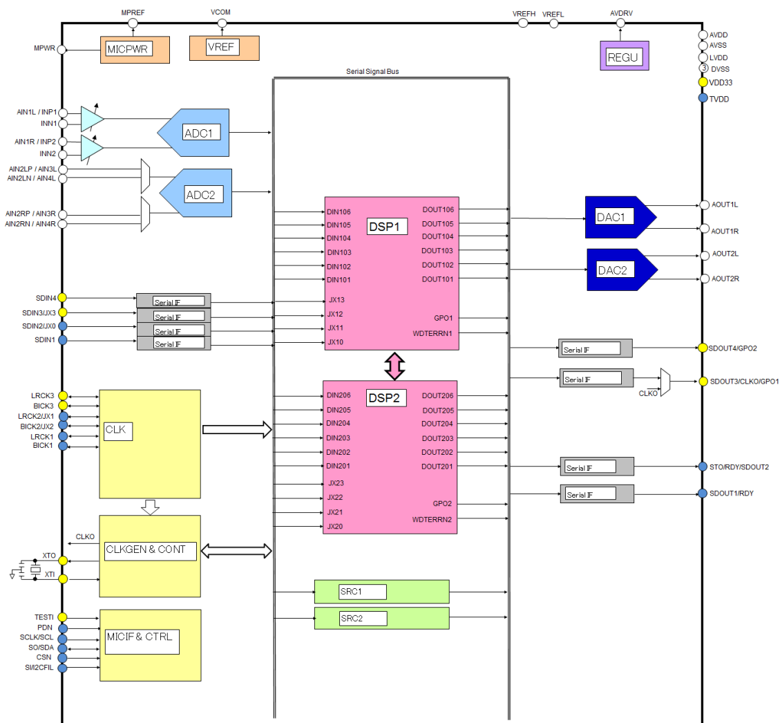
Figure 1. Block Diagram
