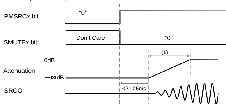
Figure 78. Soft Mute Semi-Auto Mode
