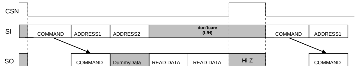
Figure 54. Echo-back Mode Reading (SPI)
