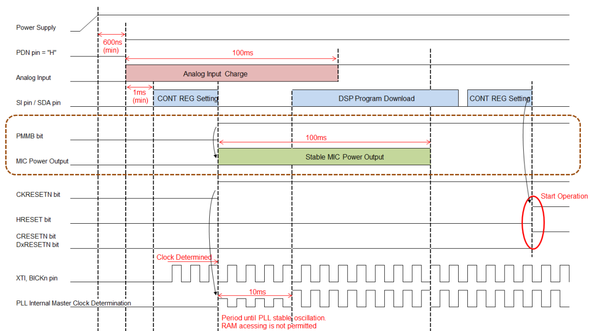
Figure 46. Power-up Sequence
