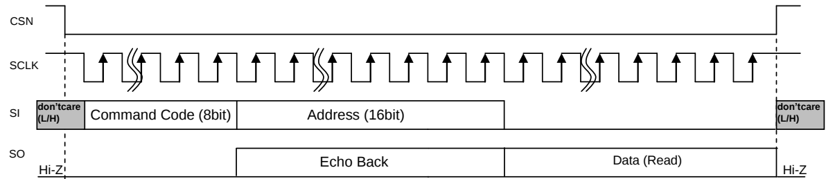
Figure 51. SPI Interface Timing (Read) (Except Command 24H, 25H, 26H and 27H)
