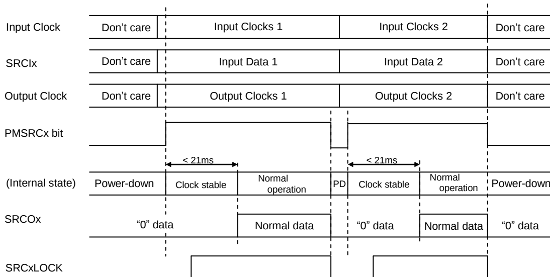
Figure 79. SRC Reset Example 1
