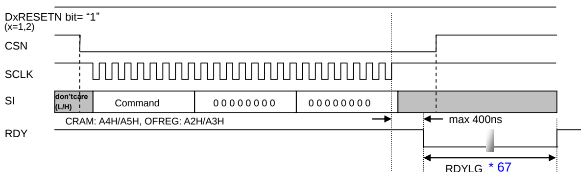
Figure 59. CRAM/OFREG Write (SPI)
