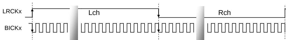
Figure 22. DSP Mode
