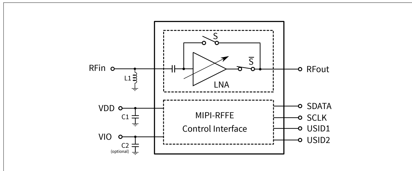
Figure 4: BGAV1A10 Application Schematic
