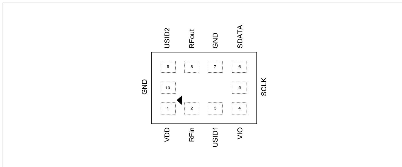
Figure 3: BGAV1A10 Pin Configuration (top view)
